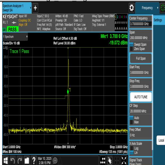
NTNV-N77-3700-3980-PC2-30-15-L-DFT-QPSK-Edge 1RB Left-Ant1-PASS
