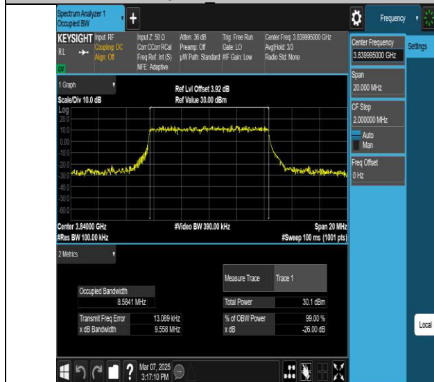
NTNV-N77-3700-3980-PC2-30-10-M-DFT-16QAM-Outer_Full-Ant1-PASS
