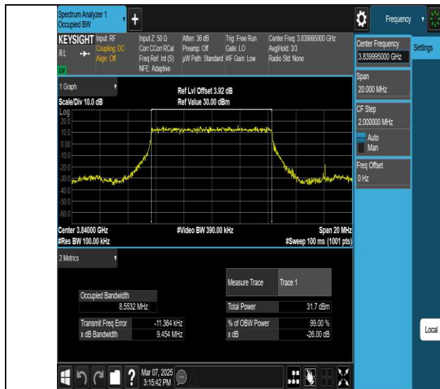
NTNV-N77-3700-3980-PC2-30-10-M-DFT-PI2BPSK-Outer_Full-Ant1-PASS
