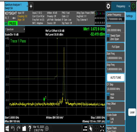
NTNV-N77-3700-3980-PC2-30-15-L-DFT-QPSK-Edge 1RB Right-Ant1-PASS
