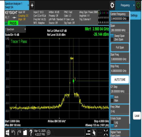
NTNV-N77-3700-3980-PC2-30-10-H-DFT-QPSK-Outer_Full-Ant1-PASS
