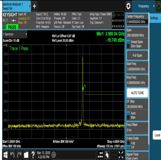
NTNV-N77-3700-3980-PC2-30-10-H-DFT-QPSK-Edge 1RB Right-Ant1-PASS
