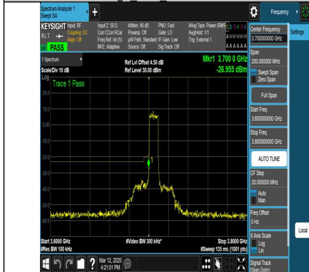
NTV-N77-3700-3980-PC2-30-10-L-DFT-QPSK-Outer_Full- Ant1-PASS
