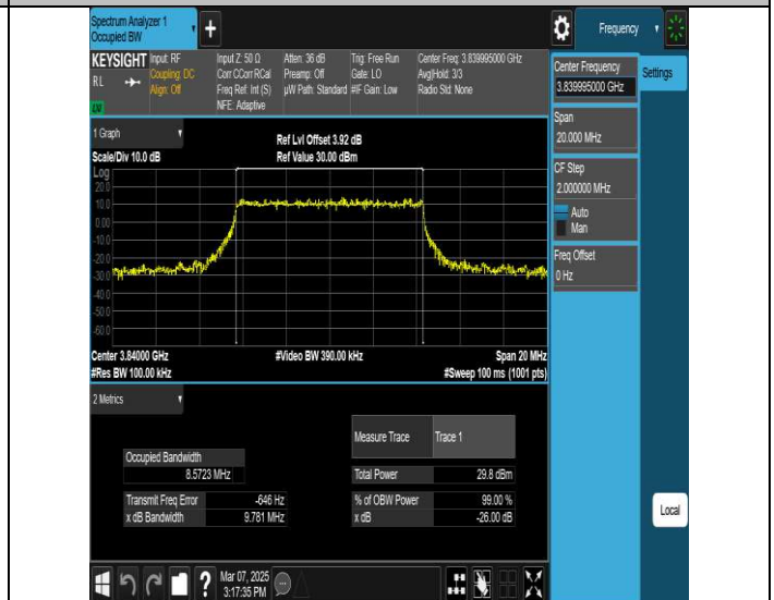
NTNV-N77-3700-3980-PC2-30-10-M-DFT-64QAM-Outer_Full-Ant1-PASS
