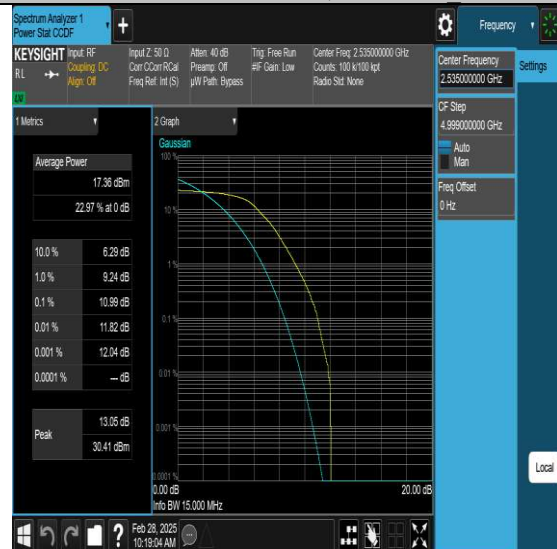
NTNV-N7-PC3-15-15-M-DFT-QPSK-Outer Full-PASS
