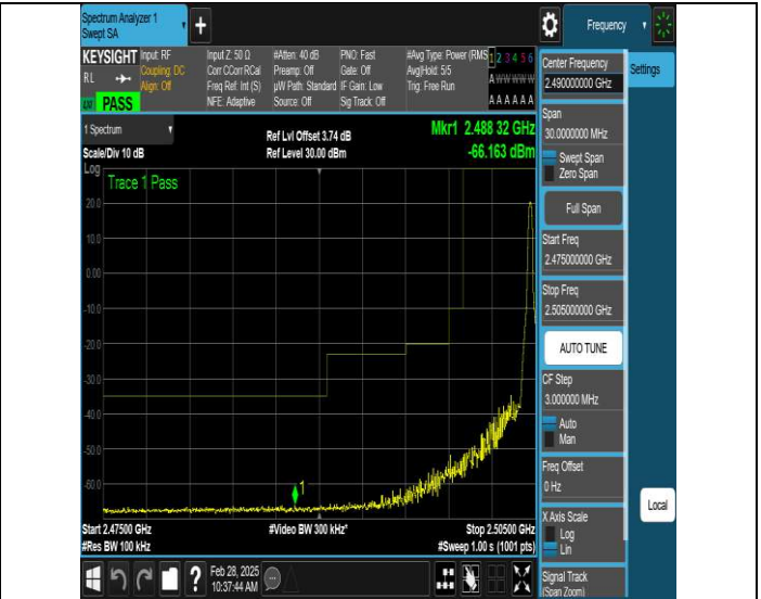
NTNV-N7-PC3-15-5-L-DFT-QPSK-Edge_1RB_Right-Ant1-PASS
