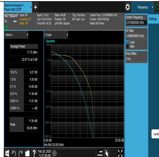
NTNV-N7-PC3-15-20-L-DFT-QPSK-Outer Full-PASS
