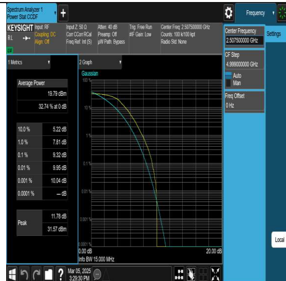
NTNV-N7-PC3-15-15-L-DFT-QPSK-Outer Full-PASS
