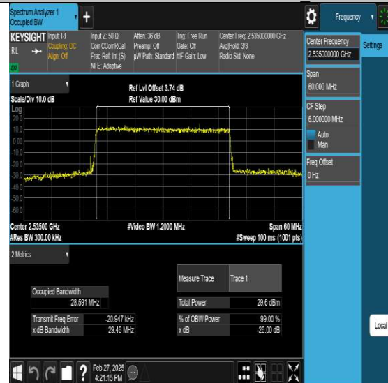
NTNV-N7-PC3-15-30-M-DFT-256QAM-Outer Full-Ant1-PASS
