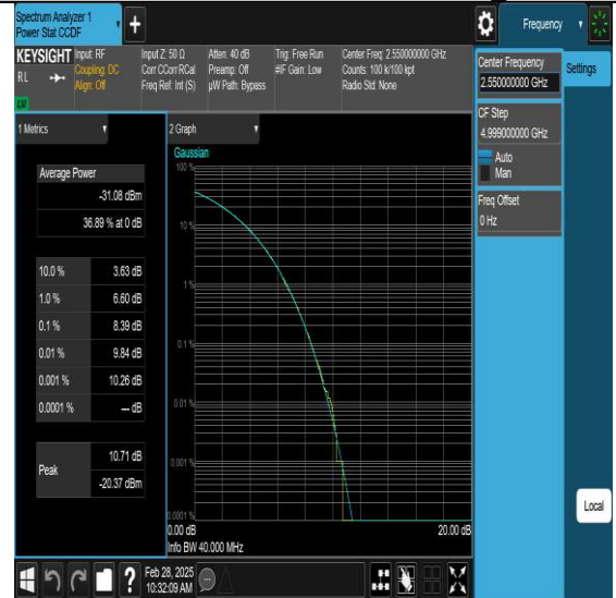
NTV-N7-PC3-15-40-H-DFT-QPSK-Outer Full-PASS
