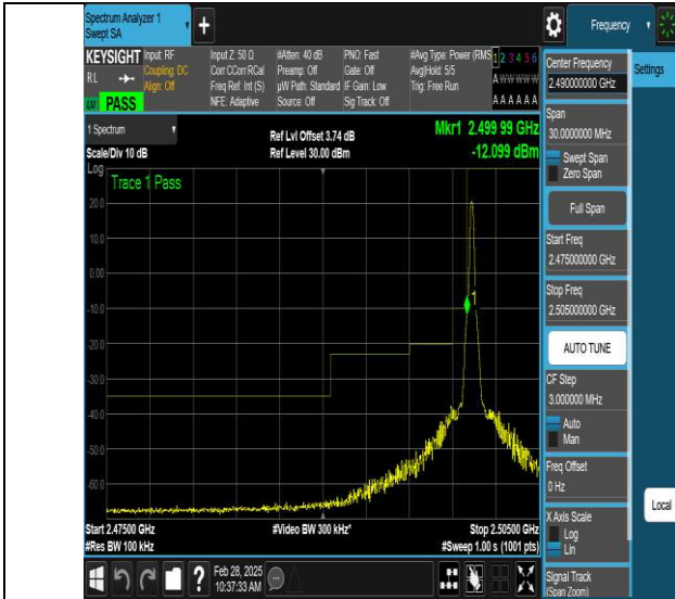
NTNV-N7-PC3-15-5-L-DFT-QPSK-Edge_1RB_Left-Ant1-PASS
