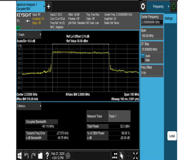
NTNV-N7-PC3-15-50-M-DFT-PI2BPSK-Outter Full-Ant1-PASS
