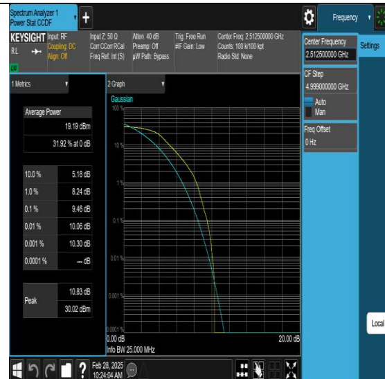
NTNV-N7-PC3-15-25-L-DFT-QPSK-Outer Full-PASS
