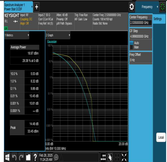
NTNV-N7-PC3-15-10-M-DFT-QPSK-Outer Full-PASS
