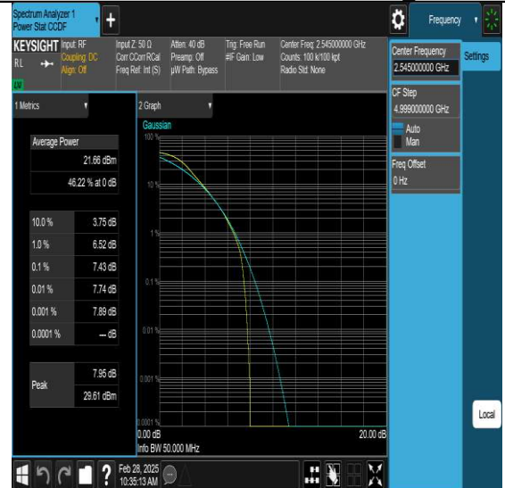
NTNV-N7-PC3-15-50-H-DFT-QPSK-Outer Full-PASS
