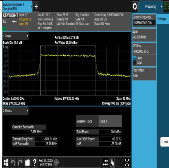
NTNV-N7-PC3-15-20-M-DFT-64QAM-Outer Full-Ant1-PASS
