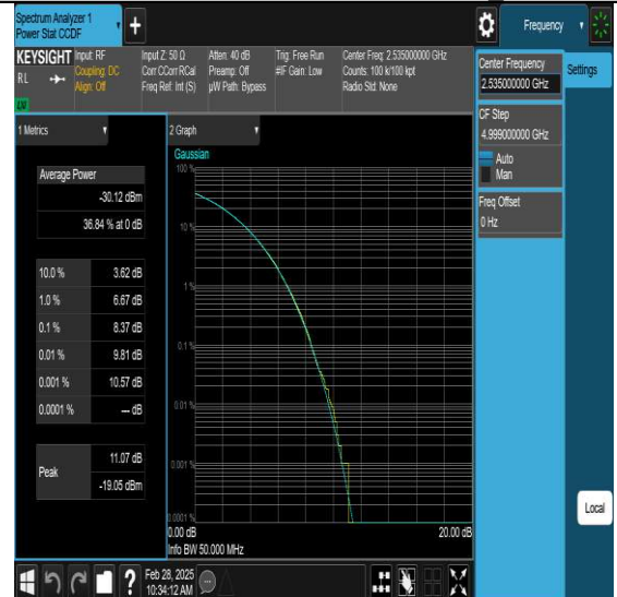
NTNV-N7-PC3-15-50-M-DFT-QPSK-Outer Full-PASS
