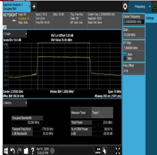
NTNV-N7-PC3-15-35-M-DFT-PI2BPSK-Outter Full-Ant1-PASS
