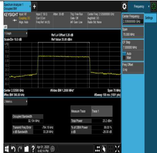
NTNV-N7-PC3-15-35-M-DFT-QPSK-Outter Full-Ant1-PASS
