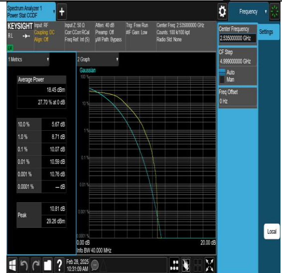
NTV-N7-PC3-15-40-M-DFT-QPSK-Outer Full-PASS
