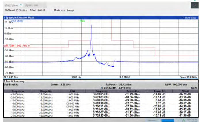
Band48-10MHz-16QAM-56690-50RB#0-PASS
