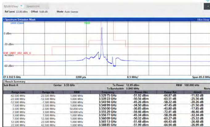
Band48-5MHz-256QAM-55265-25RB#0-PASS
