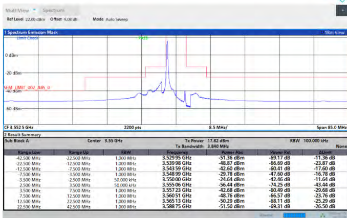
Band48-5MHz-QPSK-55265-25RB#0-PASS
