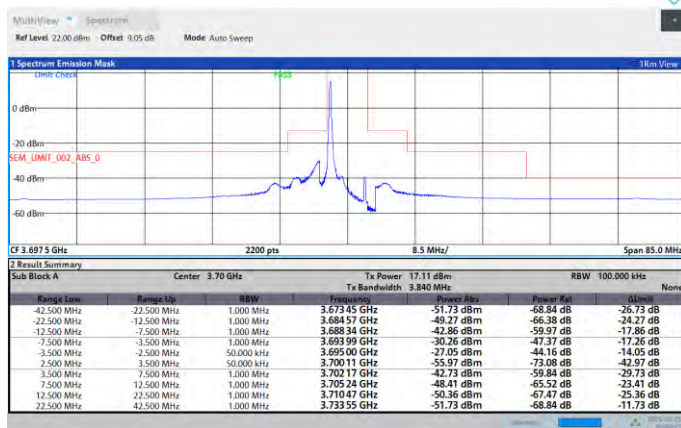
Band48-5MHz-16QAM-56715-25RB#0-PASS
