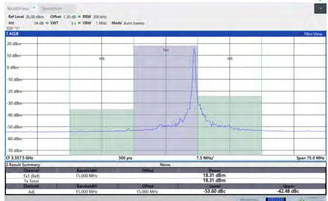
Band48-15MHz-16QAM-55990-75RB#0-PASS
