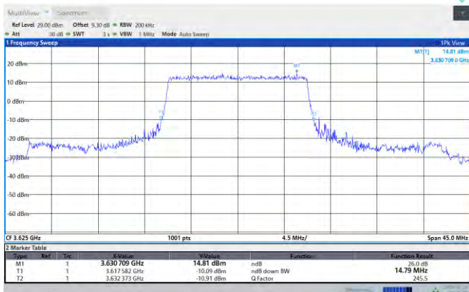
Band48-20MHz-QPSK-55990-100RB#0-PASS
