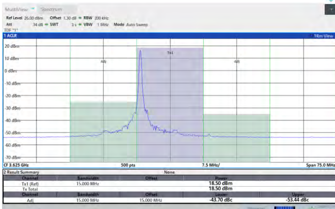
Band48-15MHz-16QAM-55990-1RB#74-PASS
