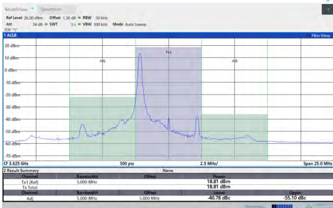
Band48-5MHz-16QAM-55990-1RB#24-PASS
