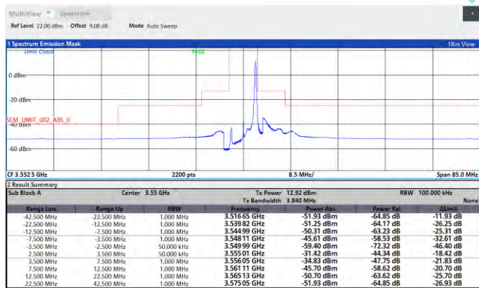
Band48-5MHz-256QAM-55990-1RB#0-PASS
