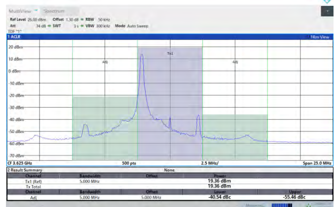
Band48-5MHz-QPSK-55990-1RB#24-PASS
