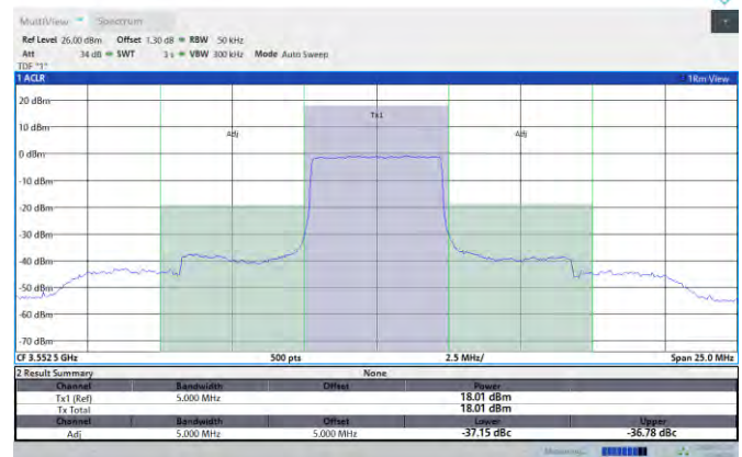
Band48-5MHz-QPSK-55990-1RB#0-PASS
