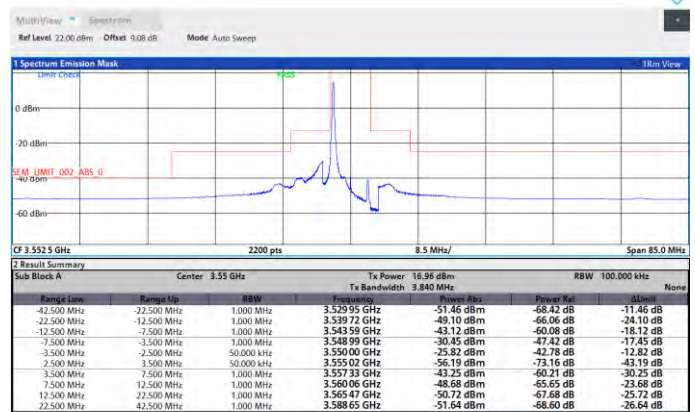
Band48-5MHz-16QAM-55265-25RB#0-PASS
