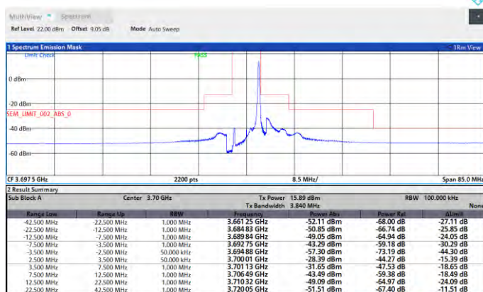
Band48-5MHz-256QAM-55265-1RB#0-PASS
