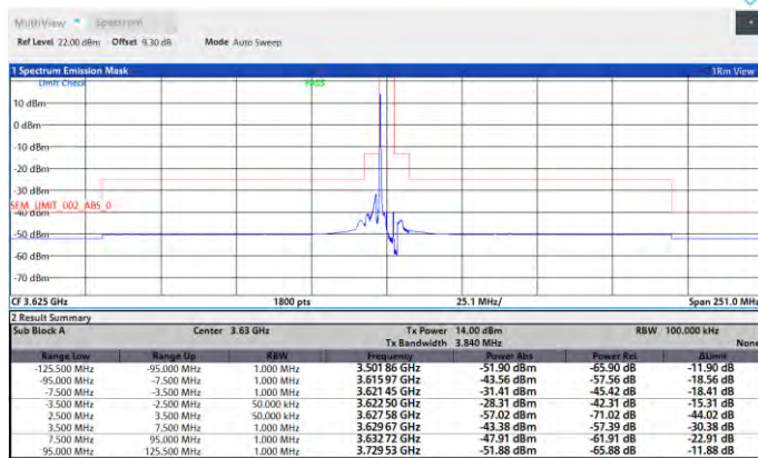
Band48-5MHz-64QAM-55990-25RB#0-PASS
