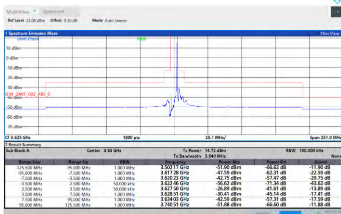
Band48-5MHz-16QAM-56715-1RB#0-PASS
