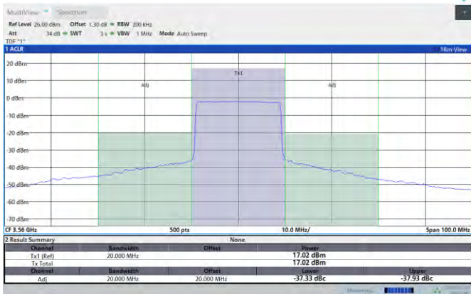
Band48-20MHz-16QAM-55990-1RB#0-PASS
