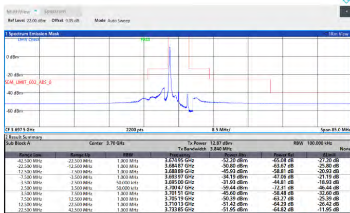
Band48-5MHz-256QAM-56715-25RB#0-PASS
