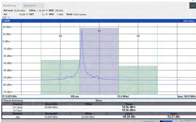
Band48-20MHz-16QAM-55990-1RB#99-PASS
