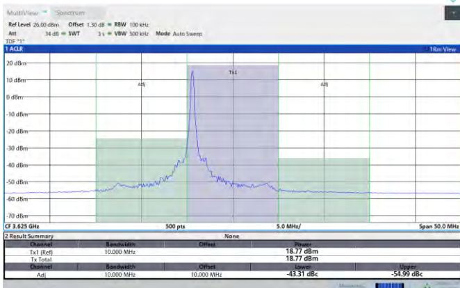
Band48-10MHz-16QAM-55990-1RB#49-PASS
