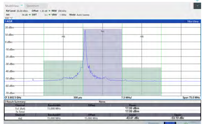
Band48-15MHz-16QAM-56665-1RB#74-PASS
