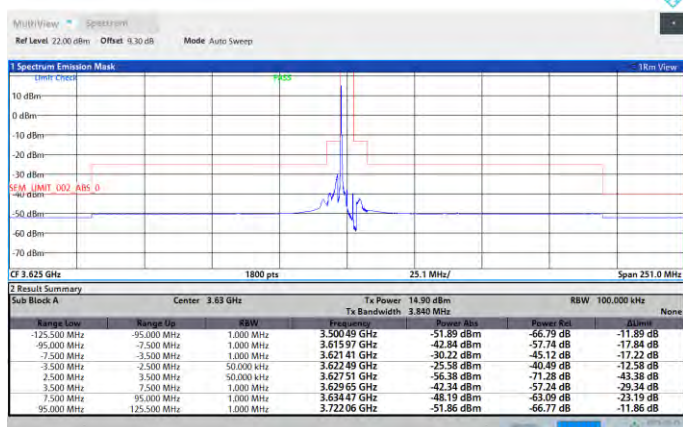
Band48-5MHz-16QAM-55990-25RB#0-PASS
