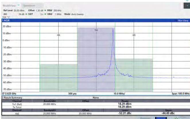
Band48-20MHz-16QAM-56640-100RB#0-PASS
