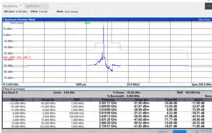
Band48-10MHz-16QAM-55990-50RB#0-PASS
