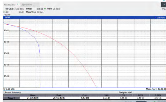
Band48-20MHz-QPSK-56640-100RB#0-PASS
