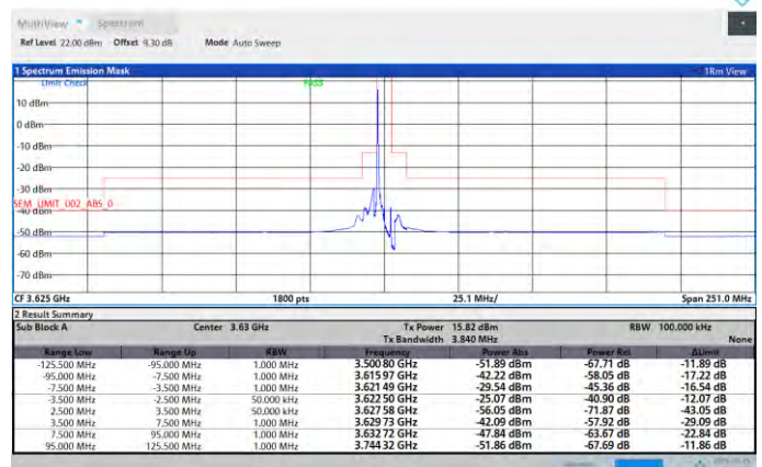
Band48-5MHz-QPSK-55990-25RB#0-PASS
