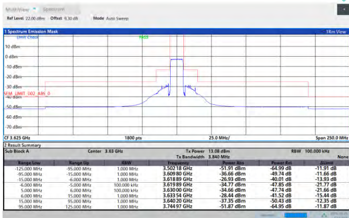
Band48-10MHz-16QAM-56690-1RB#49-PASS
