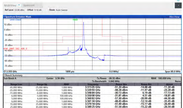
Band48-10MHz-16QAM-55290-50RB#0-PASS
