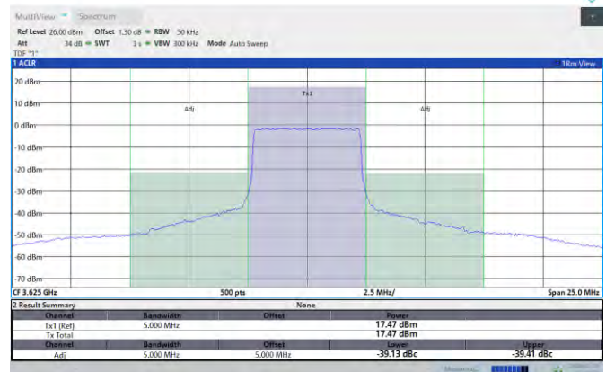
Band48-5MHz-16QAM-56715-1RB#0-PASS
