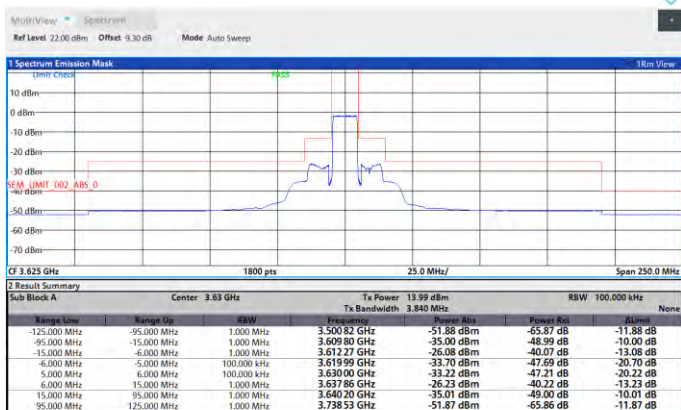
Band48-10MHz-16QAM-55290-1RB#49-PASS
