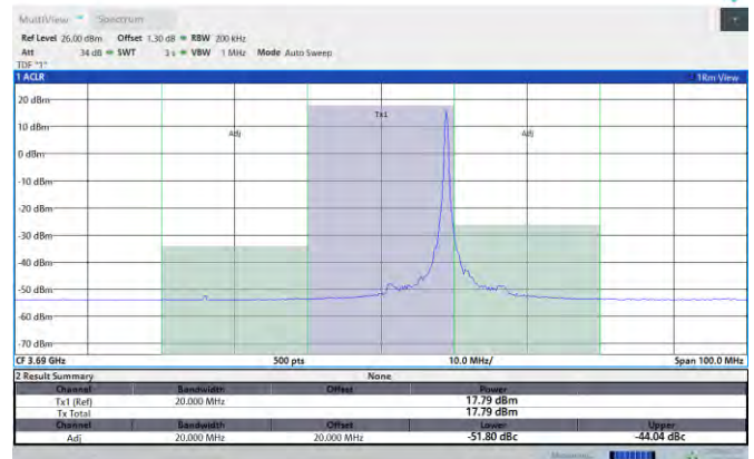
Band48-20MHz-16QAM-56640-1RB#99-PASS
