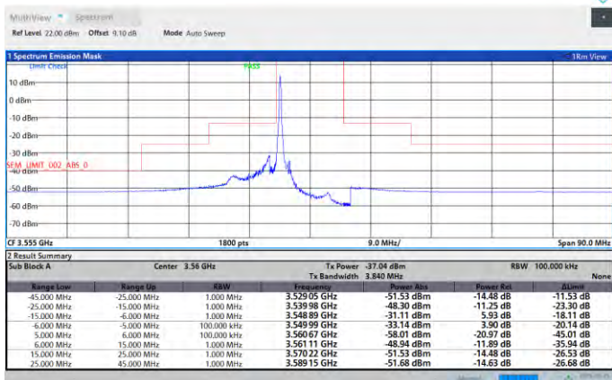
Band48-10MHz-64QAM-55290-50RB#0-PASS
