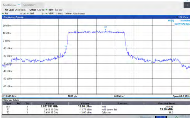
Band48-20MHz-QPSK-55990-100RB#0-PASS
