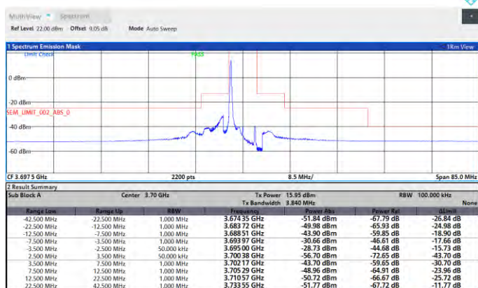
Band48-5MHz-64QAM-56715-25RB#0-PASS
