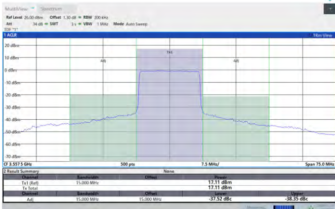
Band48-15MHz-16QAM-55990-1RB#0-PASS
