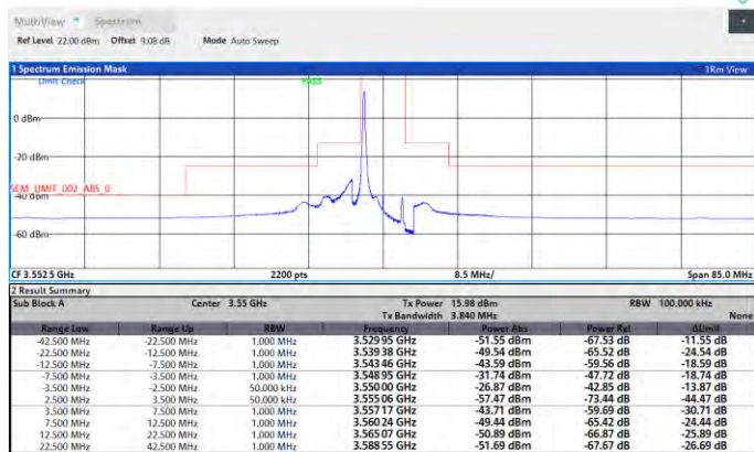
Band48-5MHz-64QAM-55265-25RB#0-PASS
