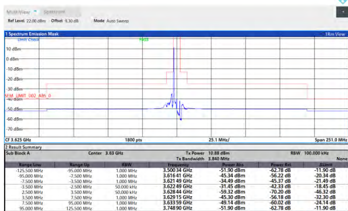
Band48-5MHz-256QAM-55990-25RB#0-PASS
