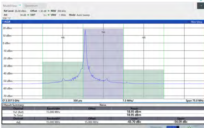
Band48-15MHz-QPSK-55315-1RB#74-PASS
