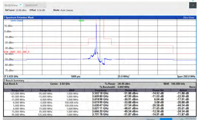
Band48-10MHz-64QAM-55990-50RB#0-PASS
