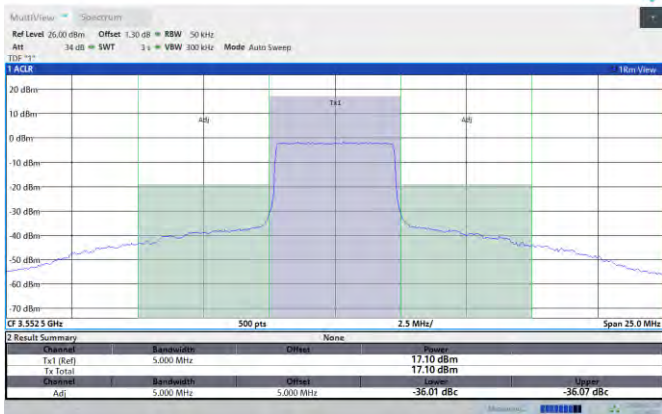
Band48-5MHz-16QAM-55990-1RB#0-PASS
