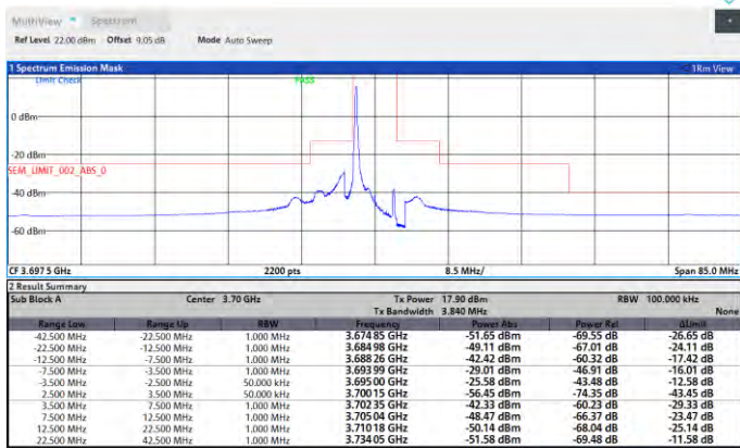
Band48-5MHz-QPSK-56715-25RB#0-PASS
