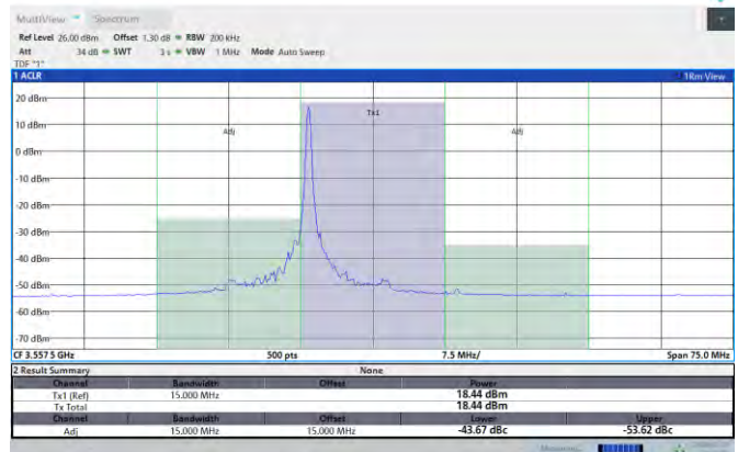
Band48-15MHz-16QAM-55315-1RB#74-PASS
