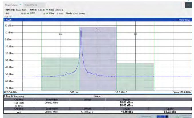
Band48-20MHz-16QAM-55340-1RB#99-PASS
