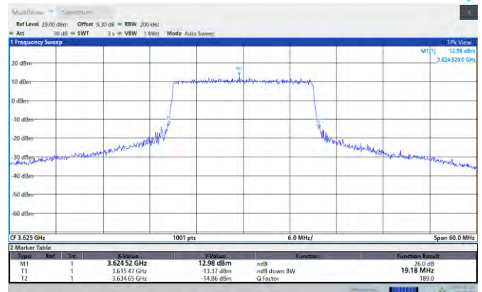
Band48-20MHz-16QAM-55990-100RB#0-PASS
