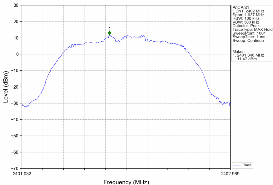
Pi/4DQPSK_2DH5_LCH_2402MHz_Ant12_NTNV
