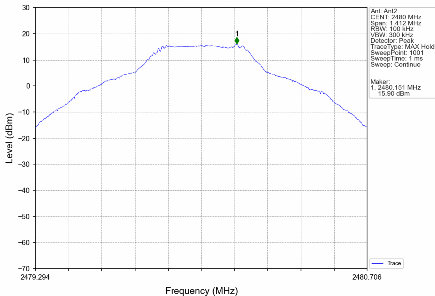
GFSK_DH5_HCH_2480MHz_Ant12_NTNV
