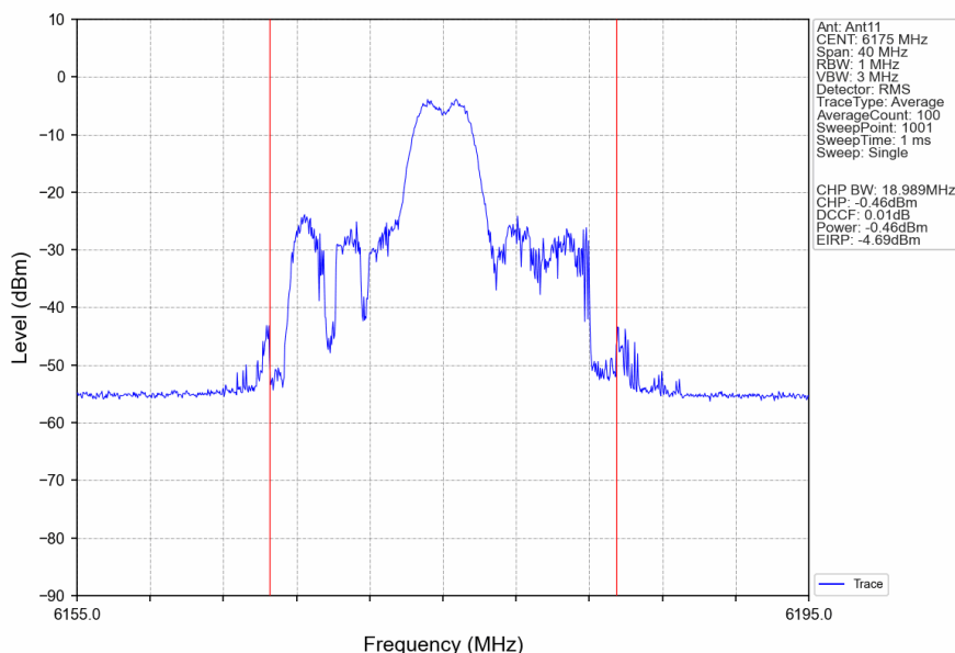
802.11ax(HEW20)_MCH_6175MHz_RU26_Mid_Ant11_NTNV
