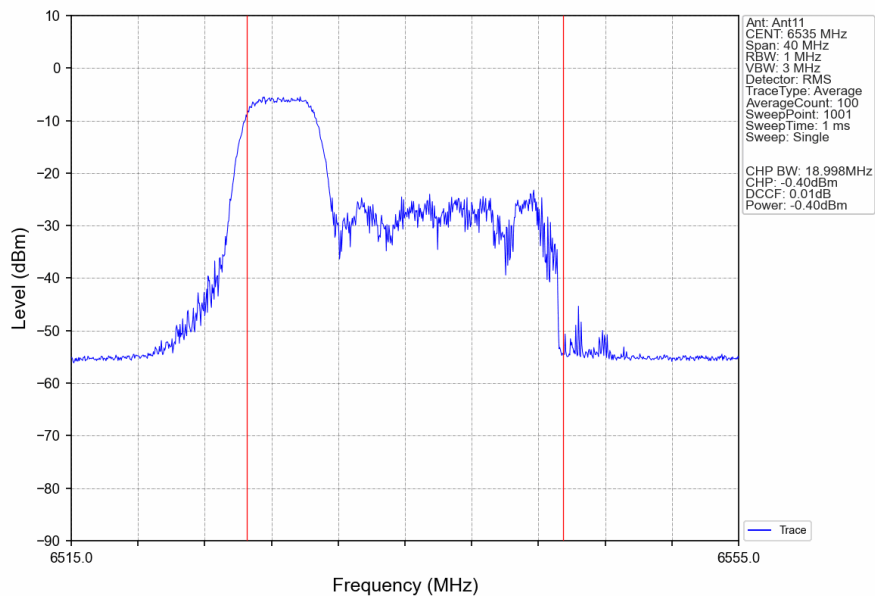
802.11ax(HEW20)_LCH_6535MHz_RU52_Left_Ant11_NTNV
