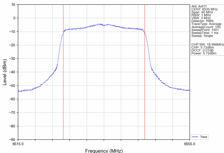
802.11ax(HEW20)_LCH_6535MHz_RU242_Left_Ant11_NTNV
