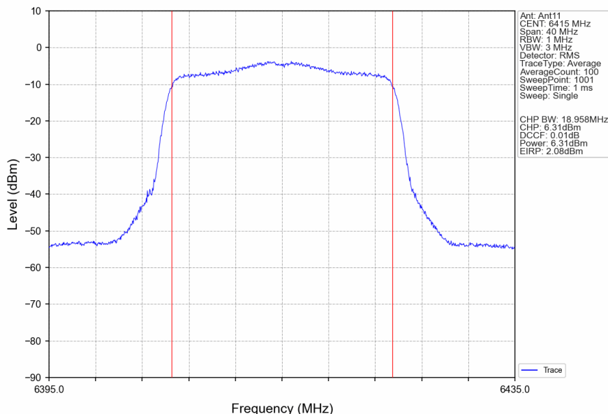
802.11ax(HEW20)_HCH_6415MHz_RU242_Left_Ant11_NTNV
