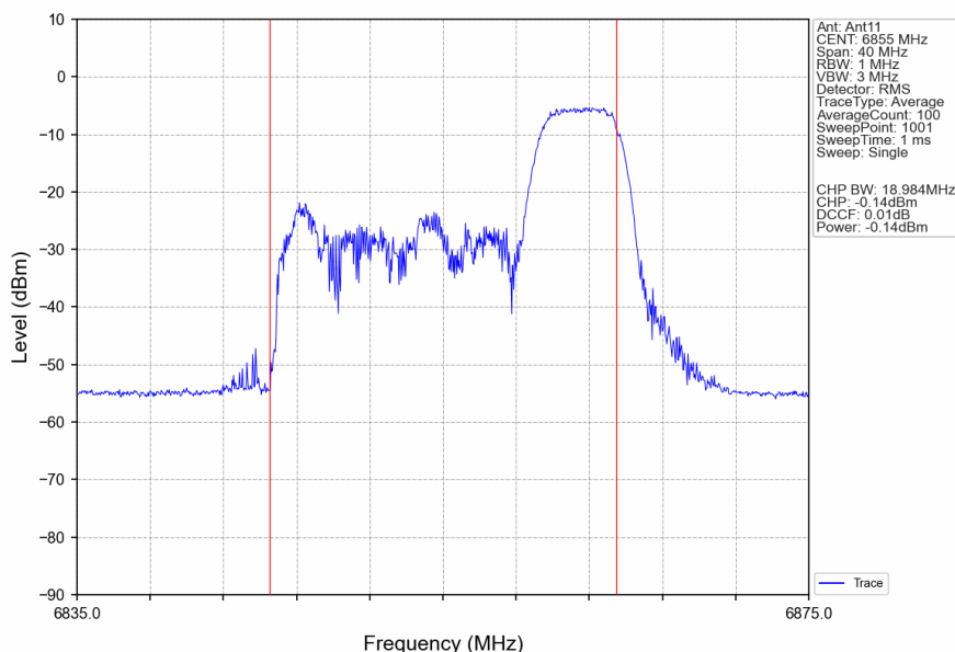
802.11ax(HEW20)_HCH_6855MHz_RU52_Right_Ant11_NTNV
