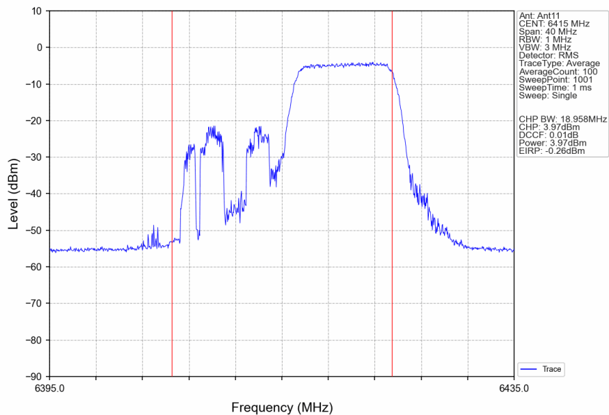
802.11ax(HEW20)_HCH_6415MHz_RU106_Right_Ant11_NTNV
