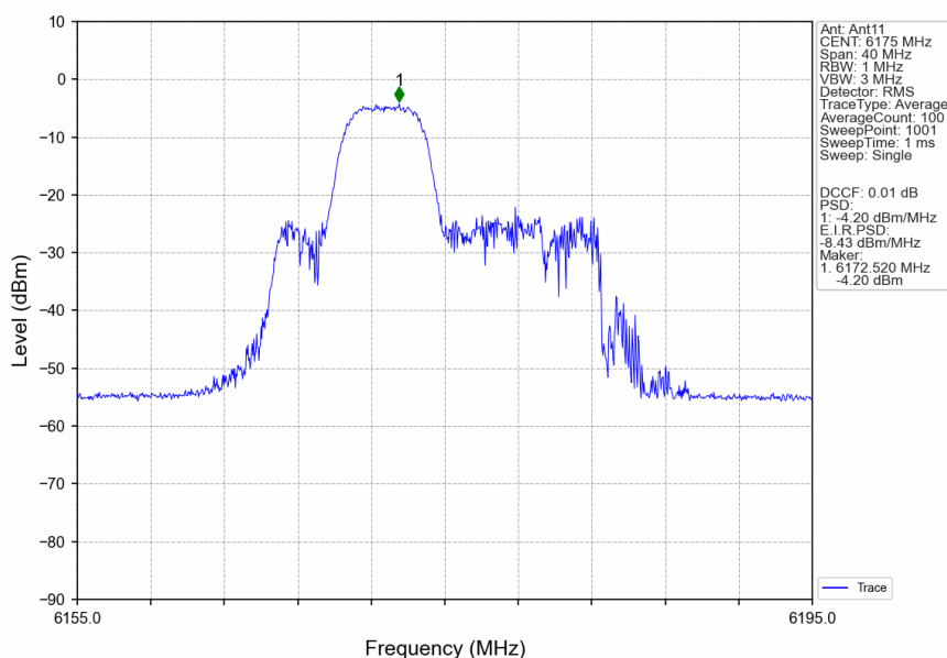
802.11ax(HEW20)_MCH_6175MHz_RU52_Mid_MIMO_NTNV
