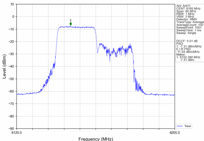
802.11ax(HEW40)_MCH_6165MHz_RU242_Left_Ant11_NTNV
