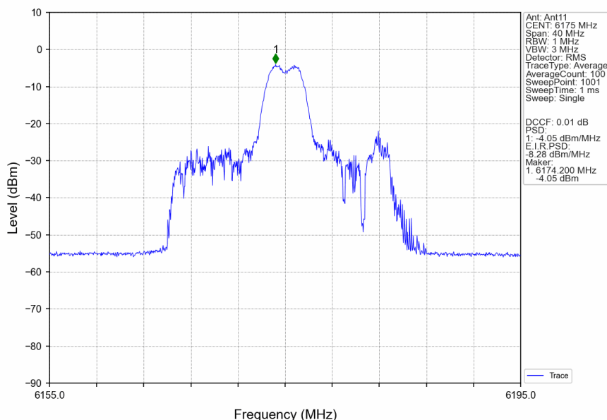
802.11ax(HEW20)_MCH_6175MHz_RU26_Mid_Ant11_NTNV
