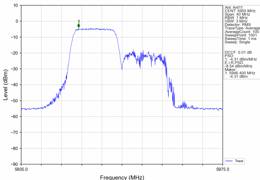
802.11ax(HEW20)_LCH_5955MHz_RU106_Left_Ant11_NTNV
