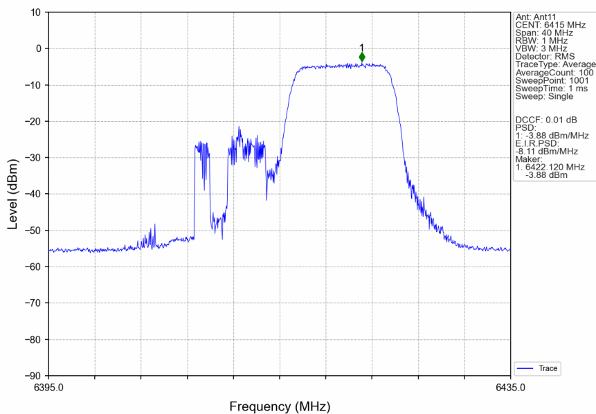
802.11ax(HEW20)_HCH_6415MHz_RU106_Right_Ant11_NTNV
