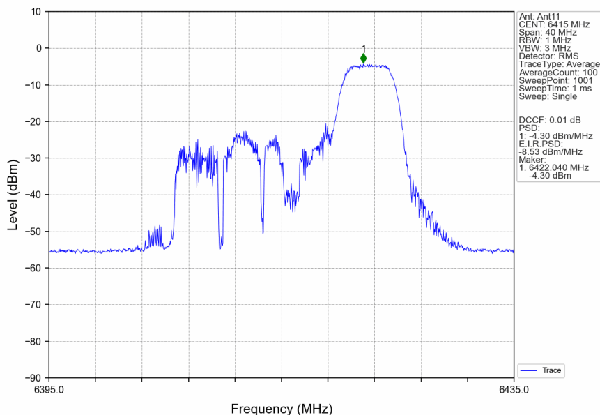
802.11ax(HEW20)_HCH_6415MHz_RU52_Right_MIMO_NTNV
