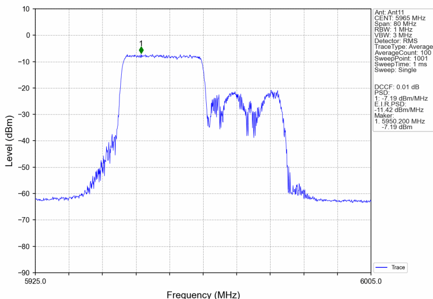
802.11ax(HEW40)_LCH_5965MHz_RU242_Left_Ant11_NTNV
