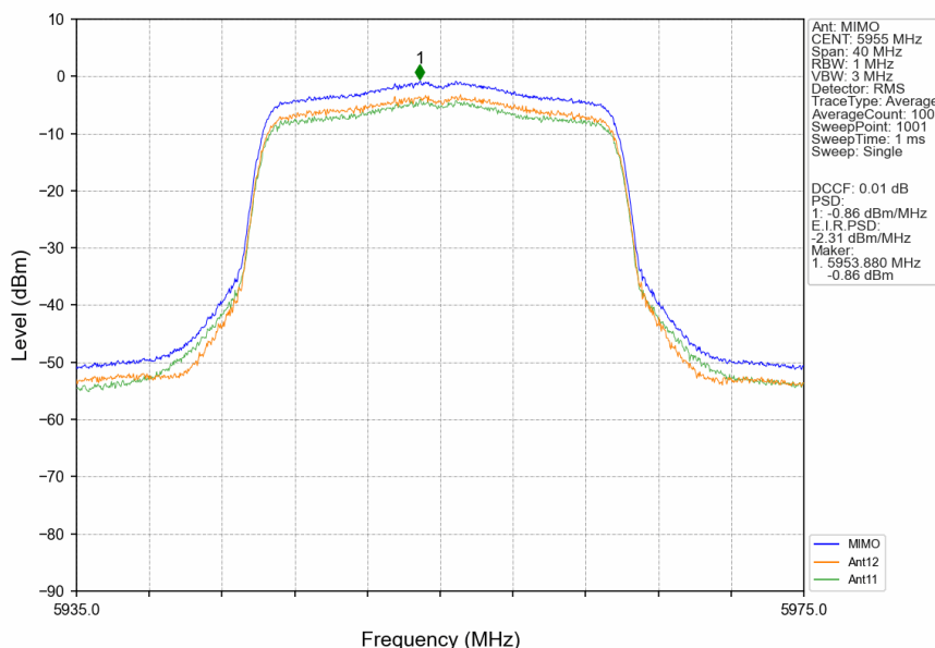
802.11ax(HEW20)_LCH_5955MHz_RU242_Left_MIMO_NTNV
