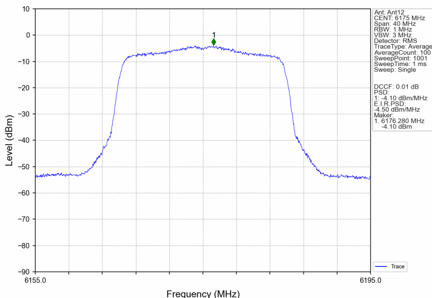
802.11ax(HEW20)_MCH_6175MHz_RU242_Left_Ant12_NTNV
