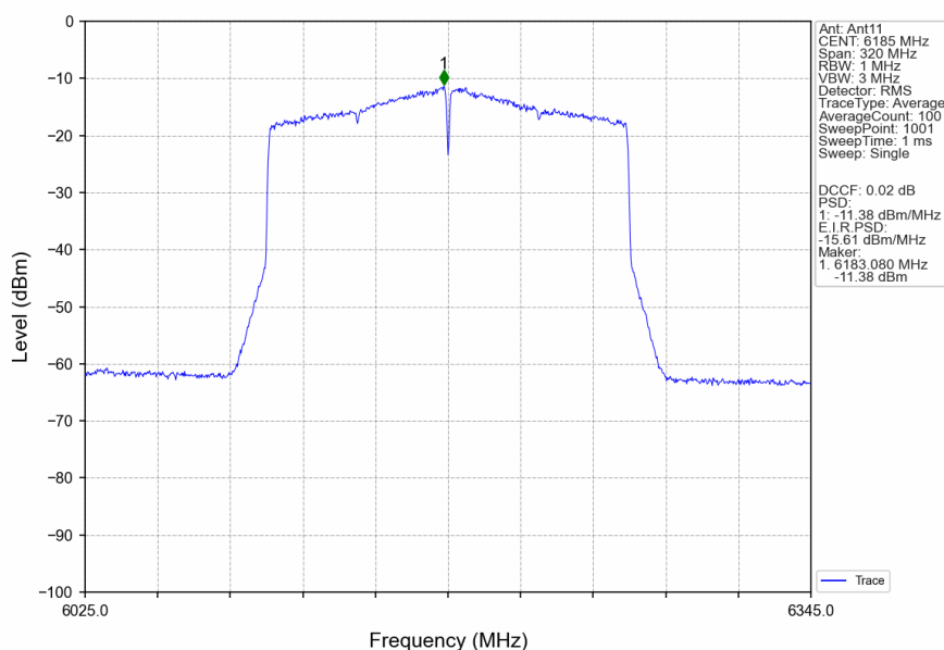
802.11ax(HEW160)_MCH_6185MHz_2xRU996_Left_MIMO_NTNV
