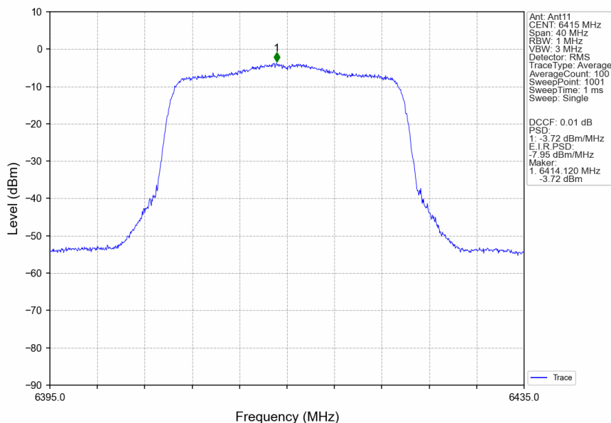
802.11ax(HEW20)_HCH_6415MHz_RU242_Left_MIMO_NTNV
