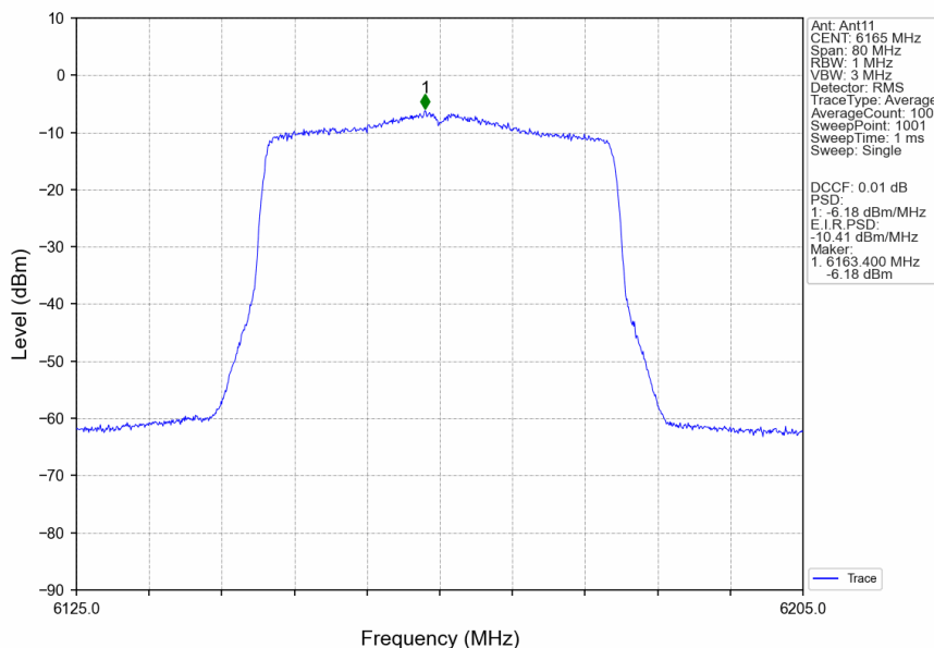
802.11ax(HEW40)_MCH_6165MHz_RU484_Left_MIMO_NTNV
