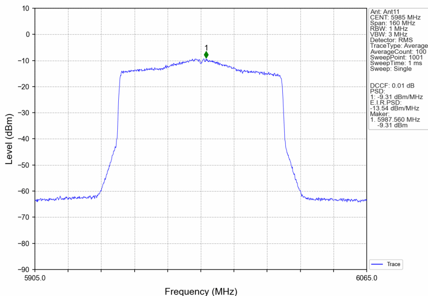
802.11ax(HEW80)_LCH_5985MHz_RU996_Left_MIMO_NTNV
