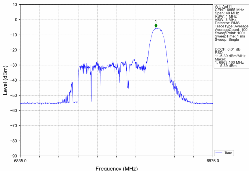
802.11ax(HEW20)_HCH_6855MHz_RU26_Right_Ant11_NTNV
