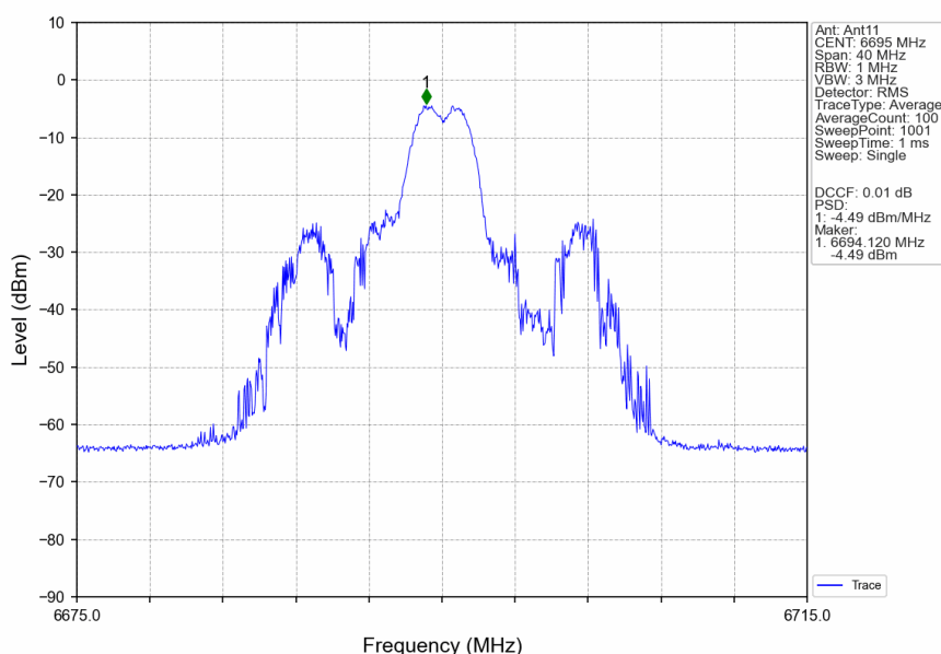
802.11ax(HEW20)_MCH_6695MHz_RU26_Mid_Ant11_NTNV
