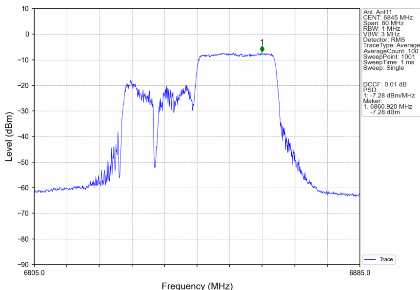
802.11ax(HEW40)_HCH_6845MHz_RU242_Right_Ant11_NTNV
