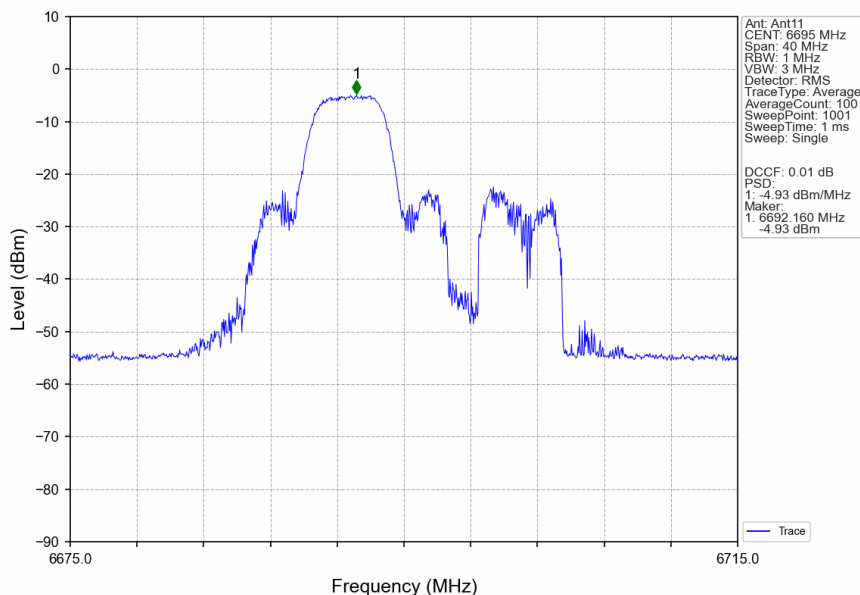
802.11ax(HEW20)_MCH_6695MHz_RU52_Mid_MIMO_NTNV
