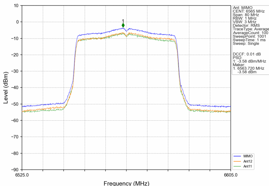
802.11ax(HEW40)_LCH_6565MHz_RU484_Left_MIMO_NTNV
