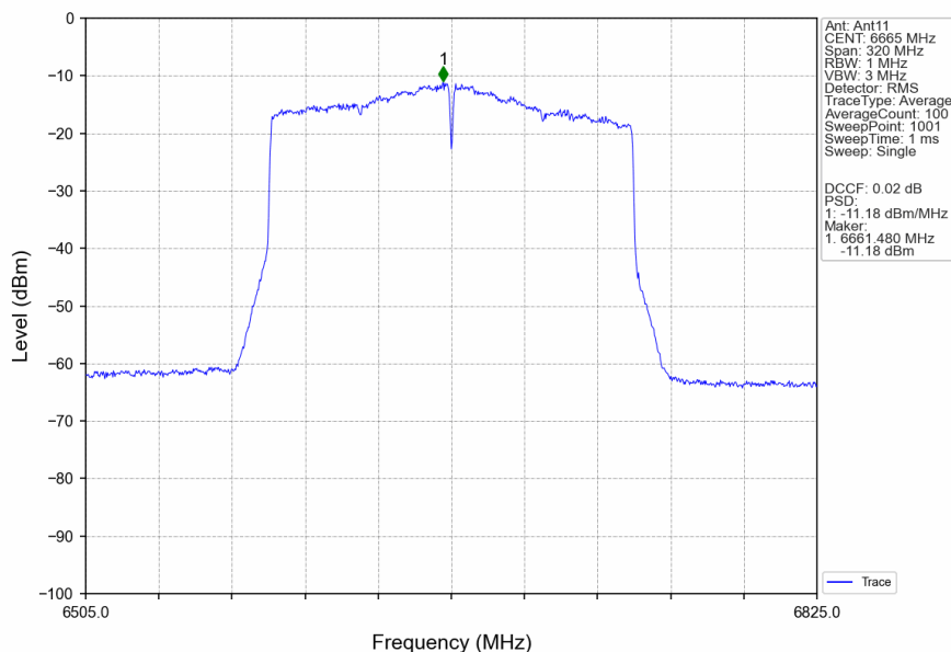
802.11ax(HEW160)_MCH_6665MHz_2xRU996_Left_MIMO_NTNV
