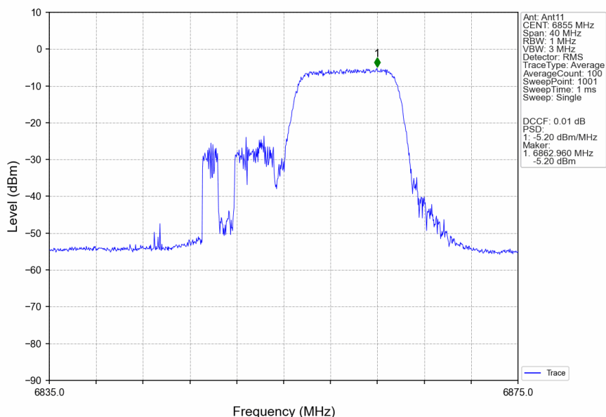
802.11ax(HEW20)_HCH_6855MHz_RU106_Right_Ant11_NTNV
