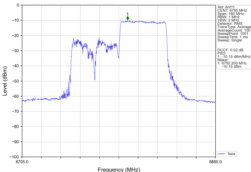
802.11ax(HEW80)_HCH_6785MHz_RU484_Right_Ant11_NTNV
