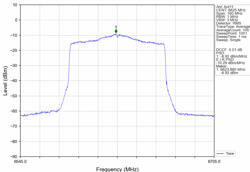
802.11ax(HEW80)_LCH_6625MHz_RU996_Left_MIMO_NTNV
