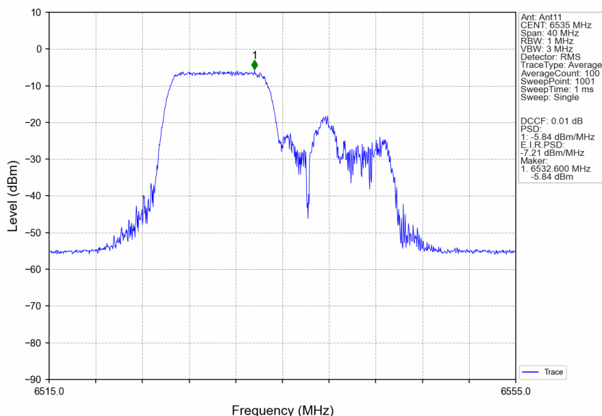
802.11ax(HEW20)_LCH_6535MHz_RU106_Left_Ant11_NTNV
