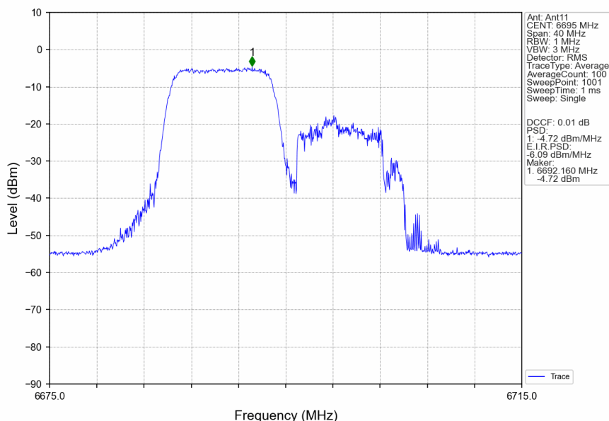
802.11ax(HEW20)_MCH_6695MHz_RU106_Left_Ant11_NTNV
