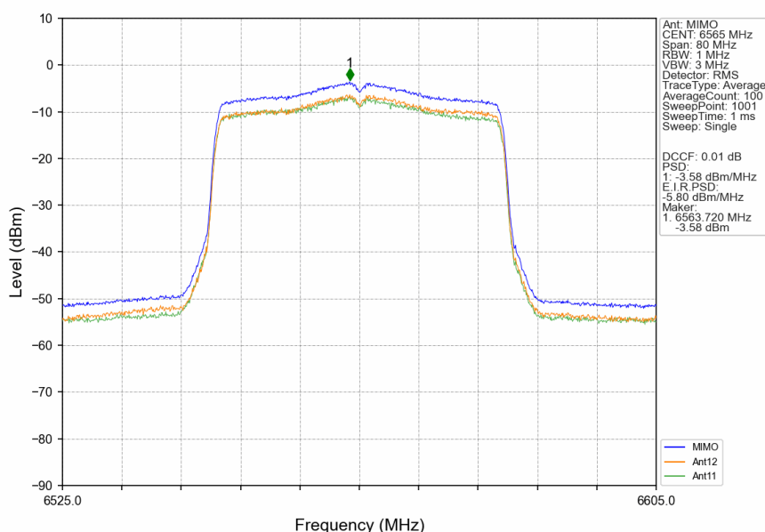
802.11ax(HEW40)_LCH_6565MHz_RU484_Left_MIMO_NTNV
