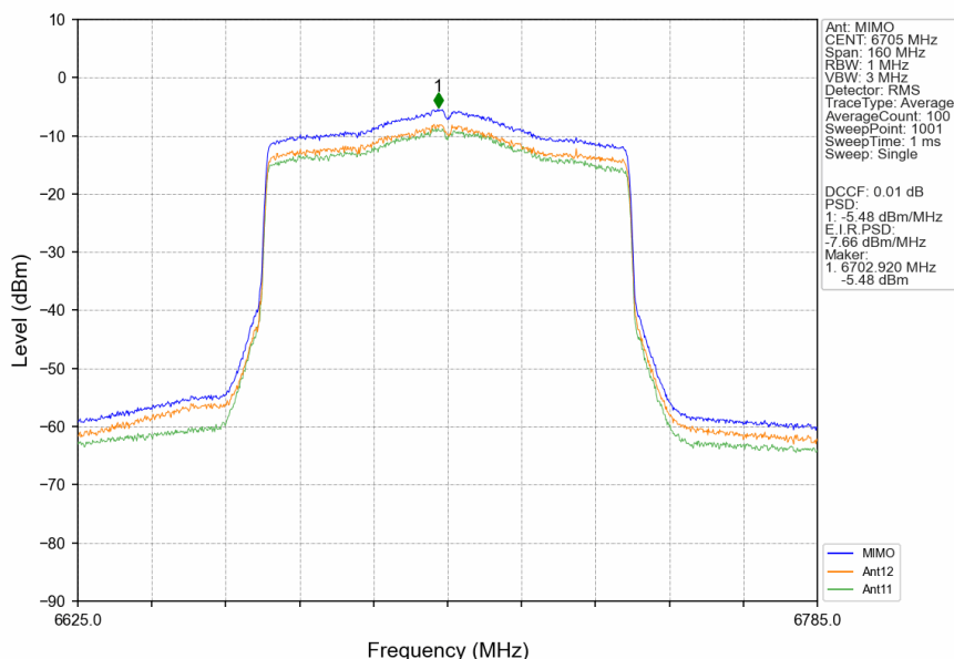
802.11ax(HEW80)_MCH_6705MHz_RU996_Left_MIMO_NTNV
