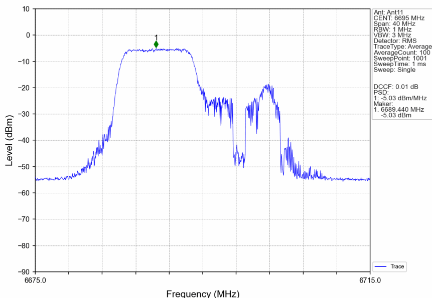
802.11ax(HEW20) MCH_6695MHz RU106 Left Ant11 NTN
