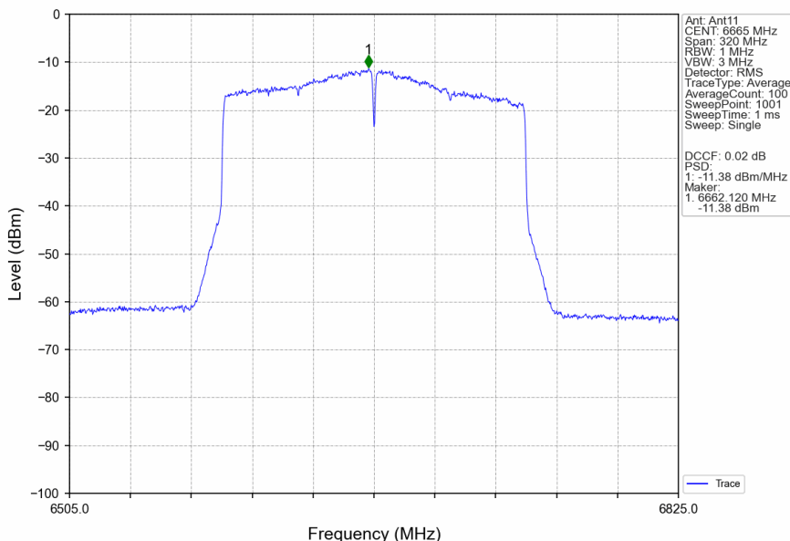
802.11ax(HEW160) MCH 6665MHz 2xRU996 Left MIMO NTNV
