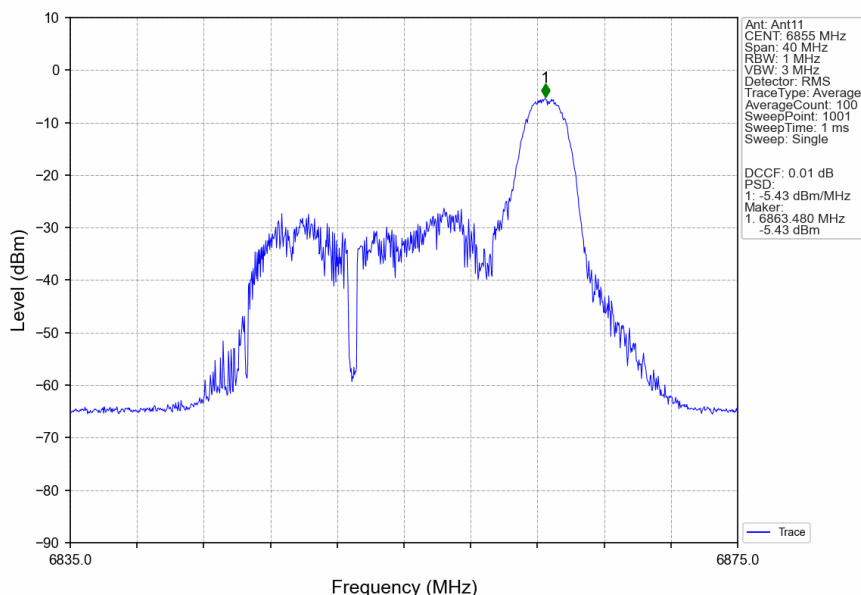
802.11ax(HEW20) HCH 6855MHz RU26 Right Ant11 NTN
