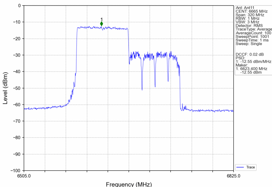
802.11ax(HEW160) MCH 6665MHz RU996 Left Ant11 NTN
