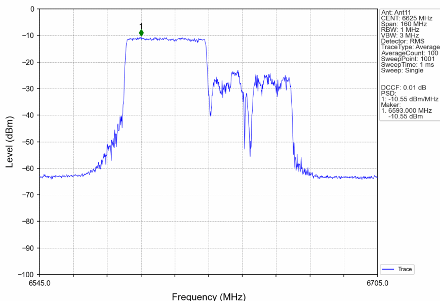
802.11ax(HEW80) LCH 6625MHz RU484 Left Ant11 NTN
