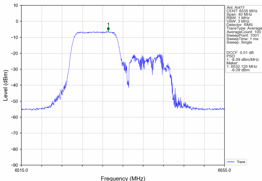
802.11ax(HEW20) LCH 6535MHz RU106 Left Ant11 NTN
