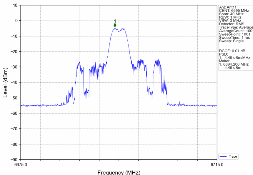
802.11ax(HEW20) MCH 6695MHz RU26 Mid Ant11 NTN
