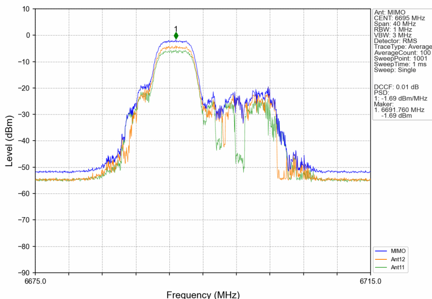
802.11ax(HEW20) MCH 6695MHz RU52 Mid MIMO NTN
