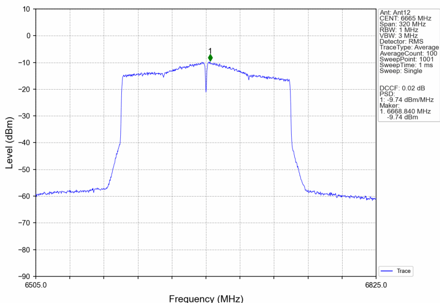
802.11ax(HEW160) MCH 6665MHz 2xRU996 Left Ant12 NTNV
