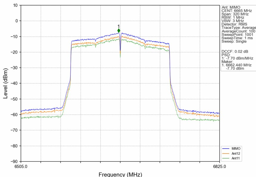
802.11ax(HEW160) MCH 6665MHz 2xRU996 Left MIMO NTNV
