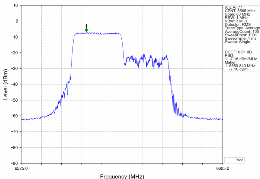
802.11ax(HEW40) LCH 6565MHz RU242 Left Ant11 NTNV
