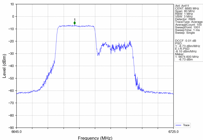
802.11ax(HEW40) MCH_6685MHz RU242 Left Ant11 NTN
