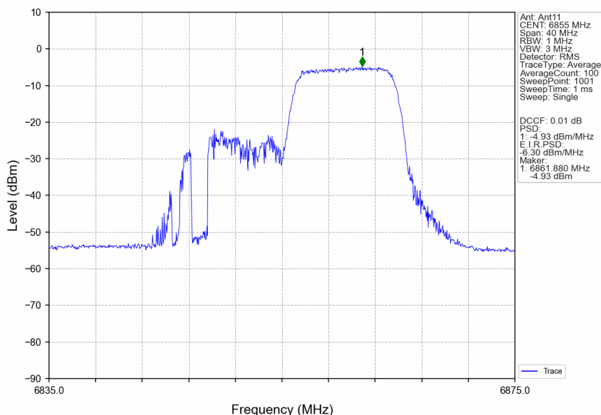
802.11ax(HEW20) HCH 6855MHz RU106 Right Ant11 NTN
