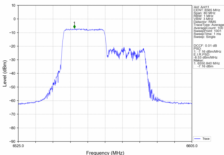
802.11ax(HEW40) LCH 6565MHz RU242 Left Ant11 NTN
