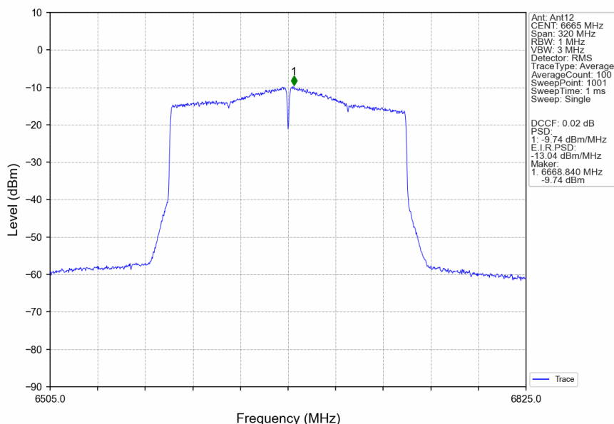
802.11ax(HEW160) MCH 6665MHz 2xRU996 Left Ant12 NTNv
