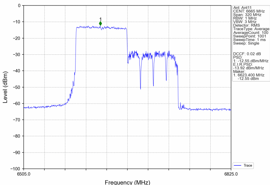
802.11ax(HEW160) MCH 6665MHz RU996 Left Ant11 NTNv
