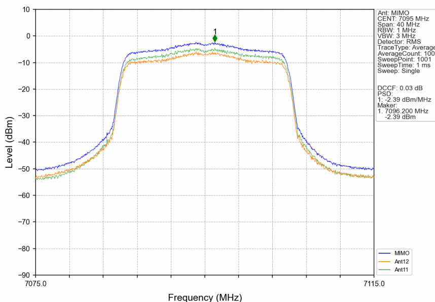
802.11ax(HEW20)_HCH_7095MHz_RU242_Left_MIMO_NTNV
