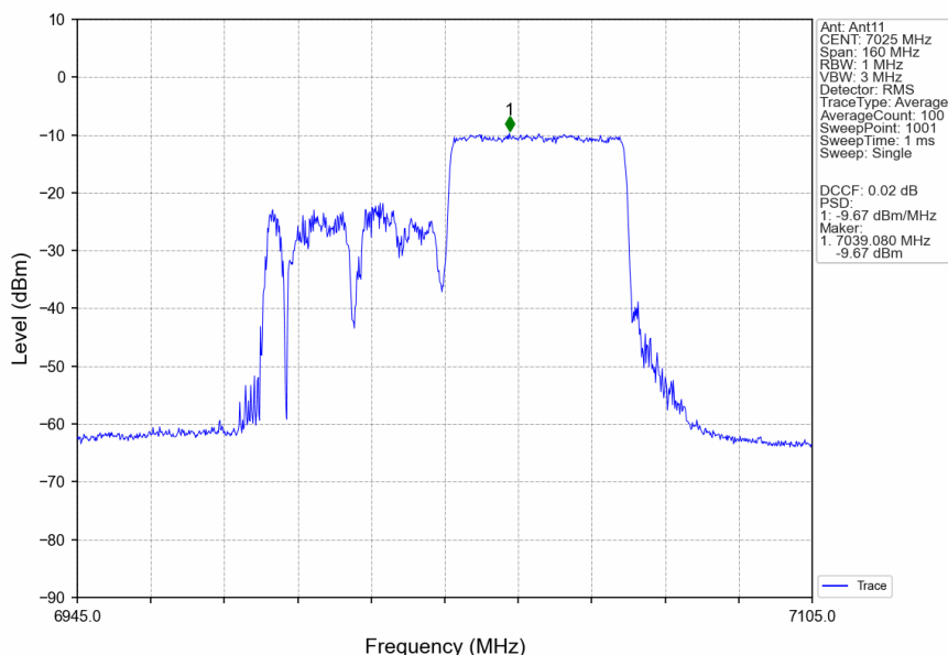
802.11ax(HEW80) HCH 7025MHz RU484 Right Ant11 NTNV
