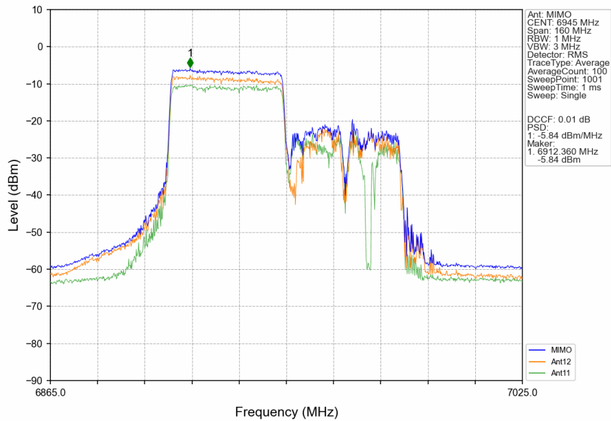
802.11ax(HEW80) LCH 6945MHz RU996 Left Ant12 NTN
