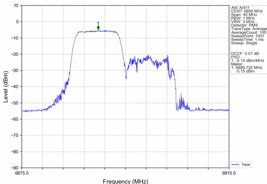
802.11ax(HEW20) LCH 6895MHz RU106 Left Ant11 NTN
