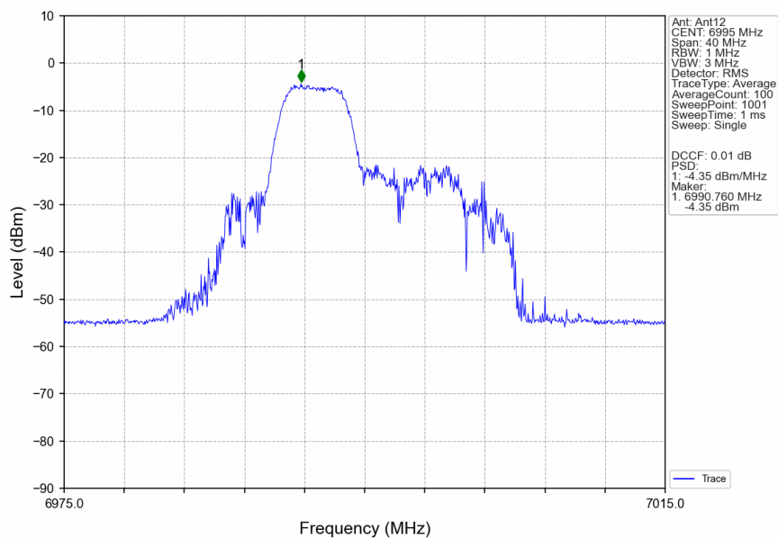
802.11ax(HEW20) MCH 6995MHz RU52 Mid Ant12 NTN
