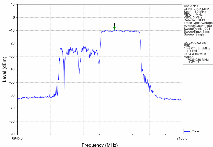
802.11ax(HEW80) HCH 7025MHz RU484 Right Ant11 NTN
