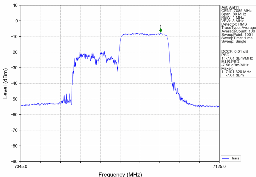
802.11ax(HEW40) HCH 7085MHz RU242 Right Ant11 NTN
