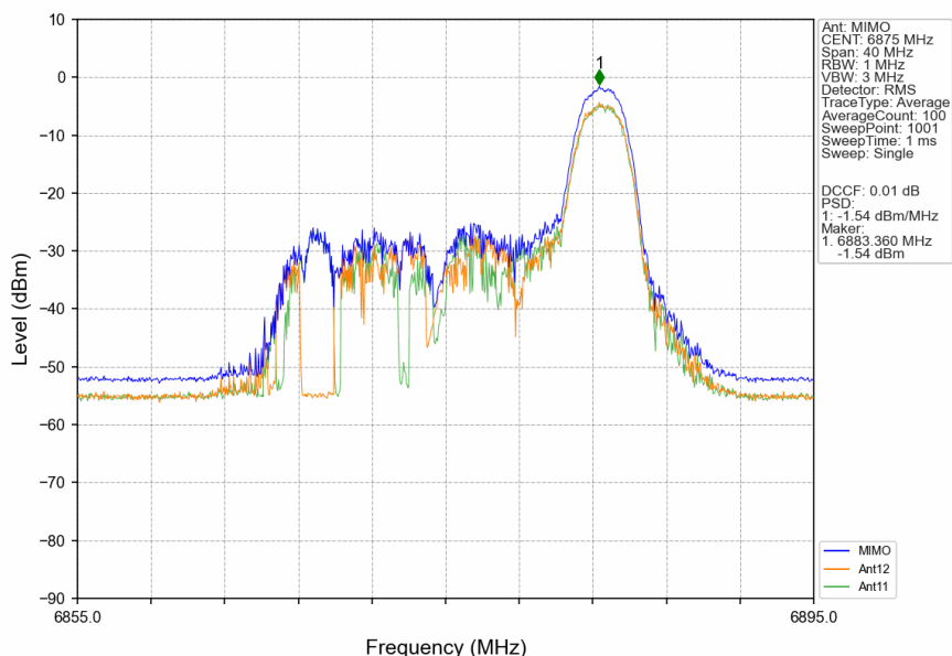
802.11ax(HEW20) HCH 6875MHz RU52 Right Ant12 NTN
