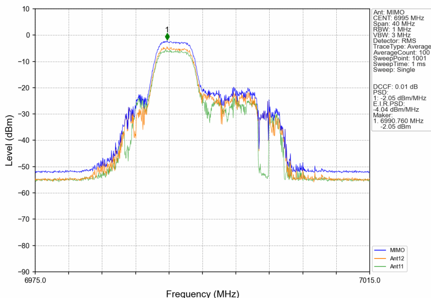
802.11ax(HEW20) MCH 6995MHz RU52 Mid MIMO NTN
