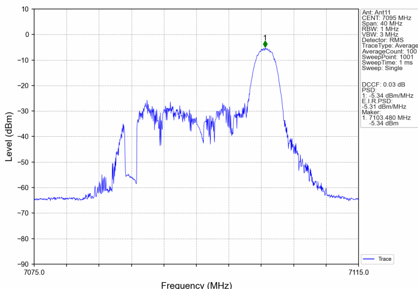
802.11ax(HEW20) HCH 7095MHz RU26 Right Ant11 NTN
