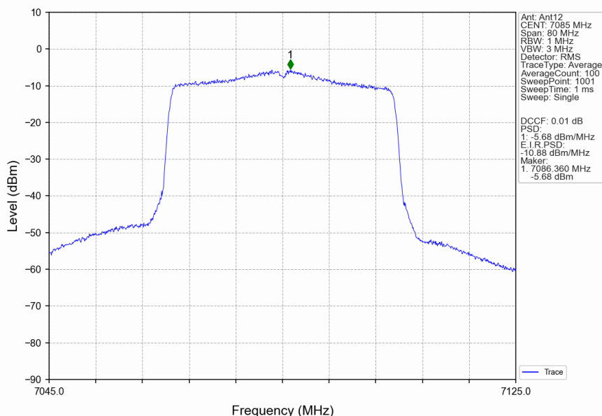
802.11ax(HEW40) HCH 7085MHz RU484 Left Ant12 NTN
