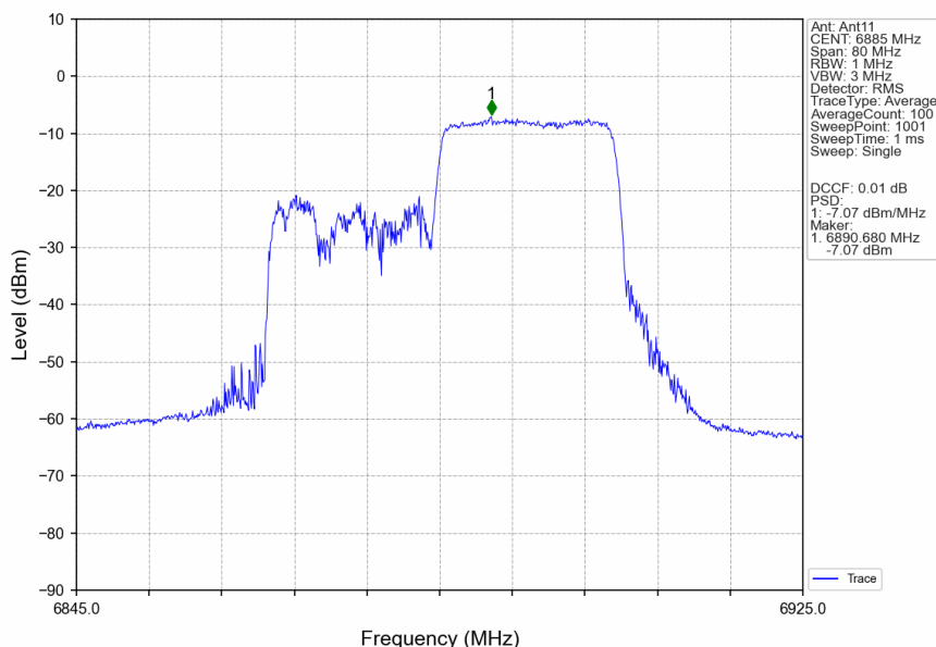
802.11ax(HEW40) HCH 6885MHz RU242 Right Ant11 NTNV
