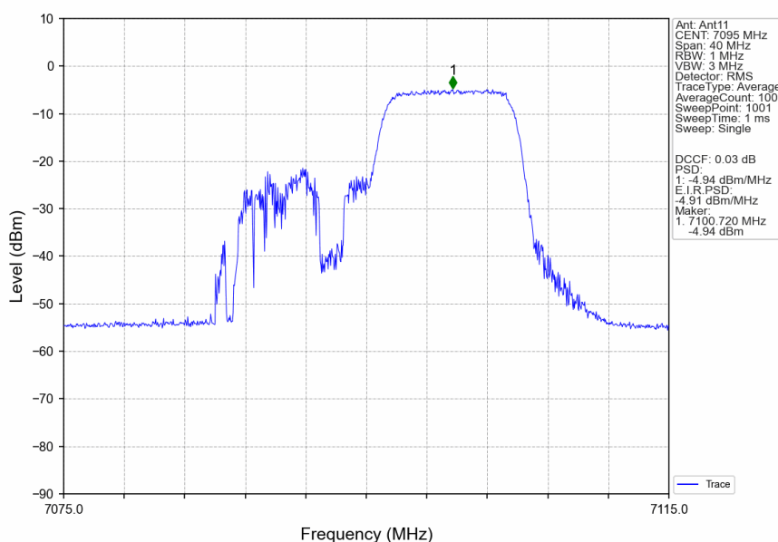
802.11ax(HEW20) HCH_7095MHz_RU106_Right_Ant11_NTNV
