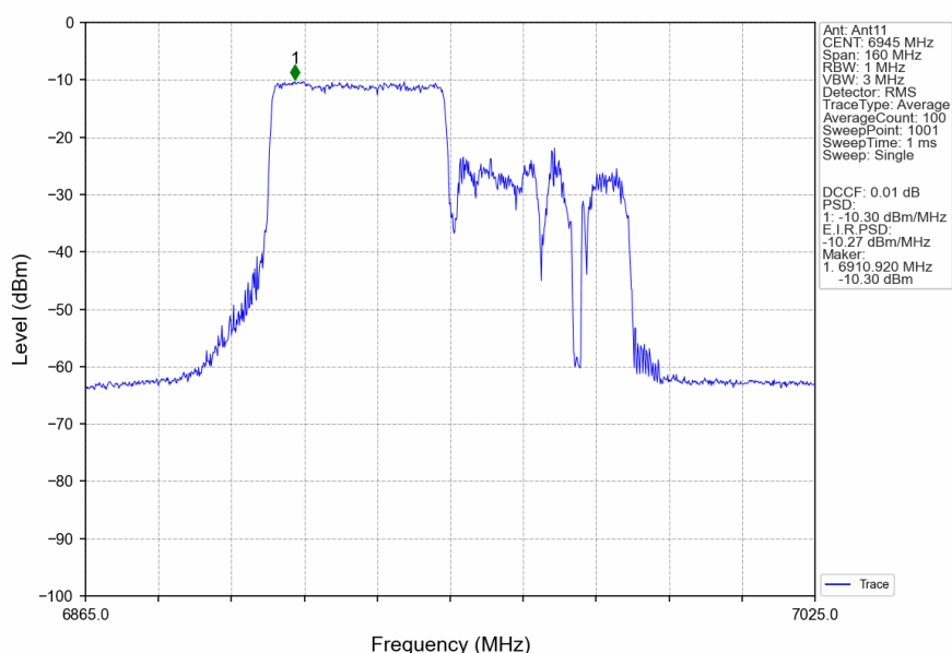
802.11ax(HEW80) LCH 6945MHz RU484 Left Ant11 NTN
