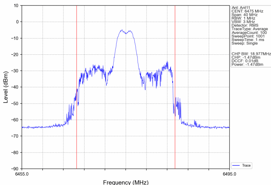
802.11ax(HEW20) MCH 6475MHz RU26 Mid Ant11 NTN
