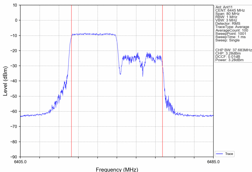
802.11ax(HEW40) LCH 6445MHz RU242 Left Ant11 NTNV
