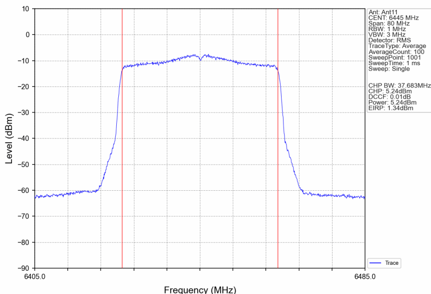
802.11ax(HEW40) LCH 6445MHz RU484 Left Ant11 NTNV
