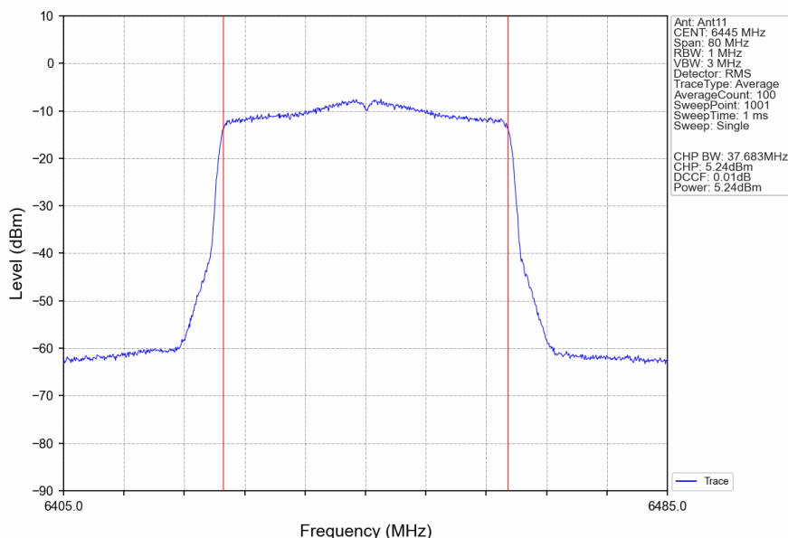
802.11ax(HEW40) LCH 6445MHz RU484 Left Ant11 NTN
