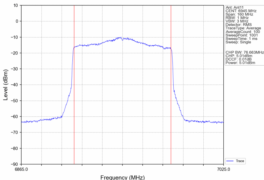
802.11ax(HEW80) LCH 6945MHz RU996 Left Ant11 NTNV
