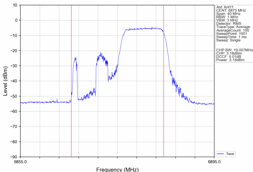
802.11ax(HEW20) HCH 6875MHz RU106 Right Ant11 NTNV
