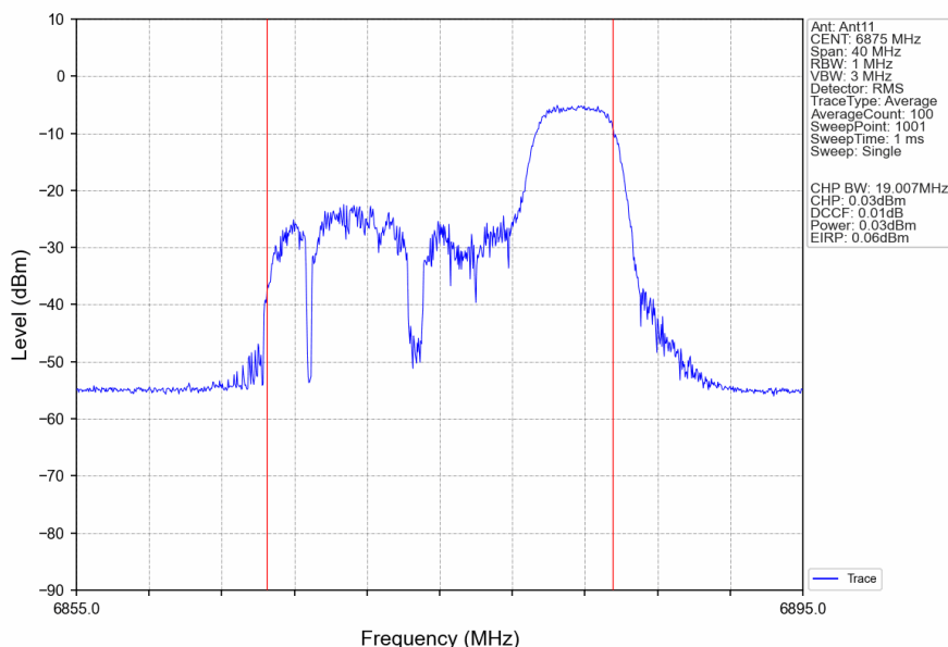
802.11ax(HEW20) HCH 6875MHz RU52 Right Ant11 NTN
