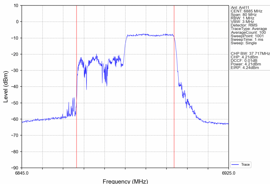
802.11ax(HEW40) HCH 6885MHz RU242 Right Ant11 NTNV
