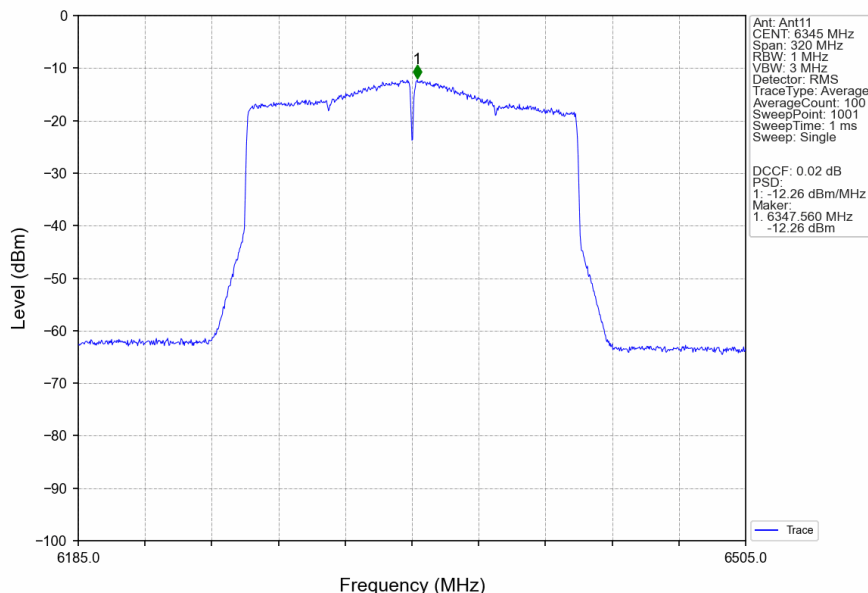
802.11ax(HEW160) HCH 6345MHz 2xRU996 Left MIMO NTVN
