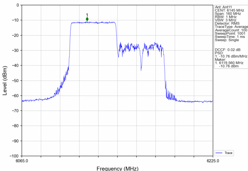
802.11ax(HEW80) MCH 6145MHz RU484 Left Ant11 NTN
