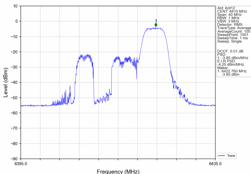
802.11ax(HEW20) HCH 6415MHz RU52 Right Ant12 NTN
