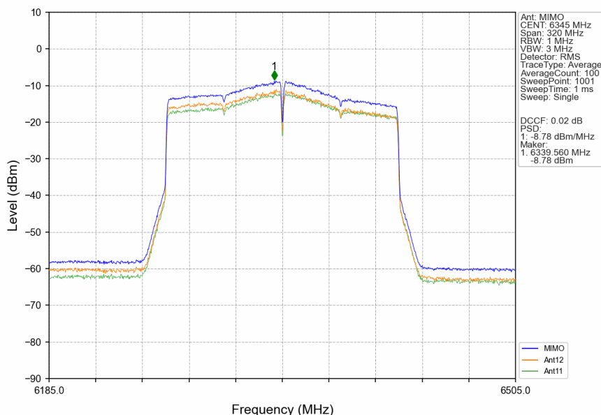
802.11ax(HEW160) HCH 6345MHz 2xRU996 Left MIMO NTVN
