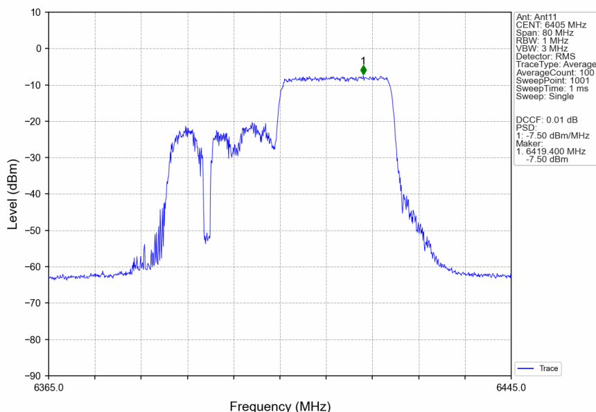
802.11ax(HEW40) HCH 6405MHz RU242 Right Ant11 NTNV
