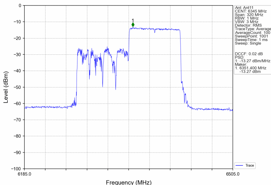
802.11ax(HEW160) HCH 6345MHz RU996 Right Ant11 NTNV
