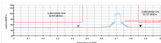
802.11ac VHT40-Channel 142: Peak
