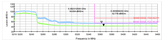
802.11ac VHT40-Channel 46: Peak + Average
