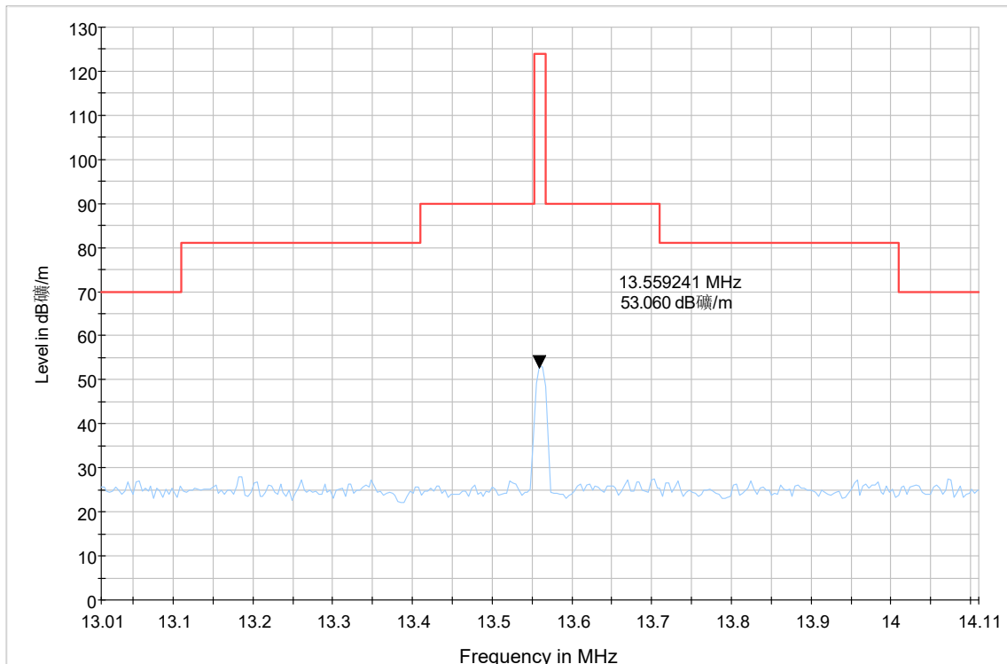
Radiates Emission from 13.01MHz to 14.11MHz
