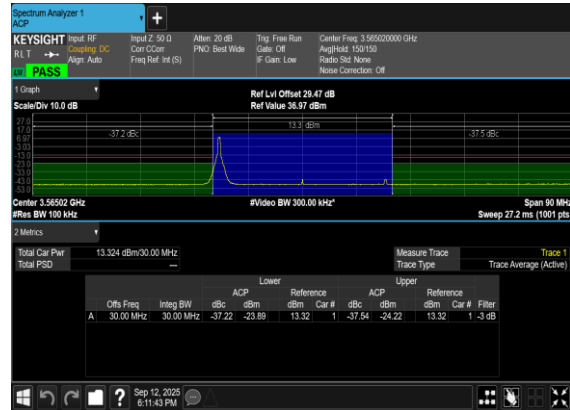
N48(30M)_DFT-s-OFDM_PI_2-BPSK_Edge_1RB_Left_Low_CH
