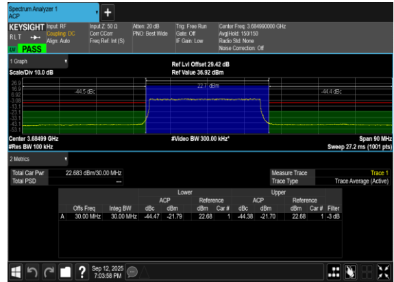
N48(30M)_DFT-s-OFDM_QPSK_Outer_Full_High_CH
