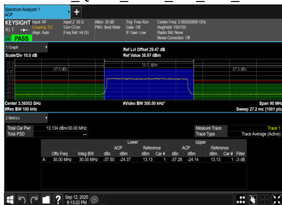
N48(30M)_DFT-s-OFDM_QPSK_Outer_Full_Low_CH
