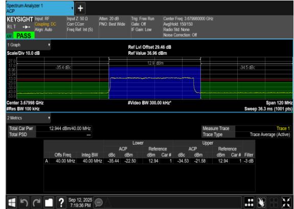
N48(40M)_DFT-s- OFDM_QPSK_Outer_Full_High_CH
