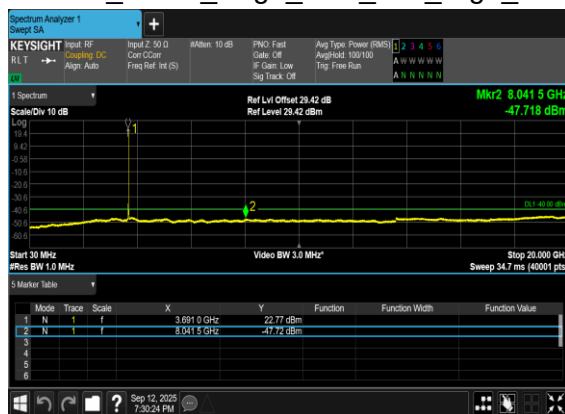
N48(10M)_DFT-s- OFDM_BPSK_Edge_1RB_Left_High_CH
