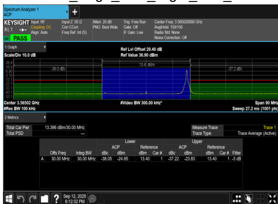
N48(30M)_DFT-s-OFDM_PI_2-BPSK_Edge_1RB_Right_Low_CH
