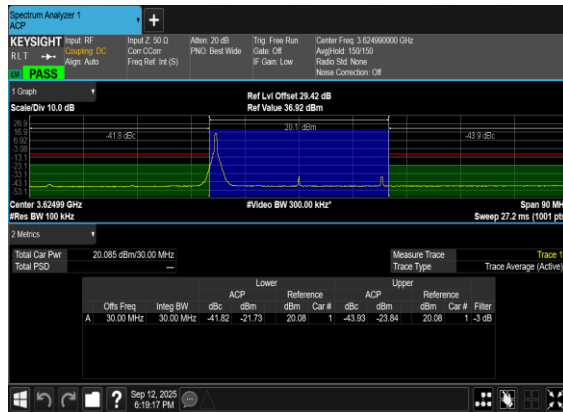
N48(30M)_DFT-s- OFDM_QPSK_Edge_1RB_Left_Mid_CH
