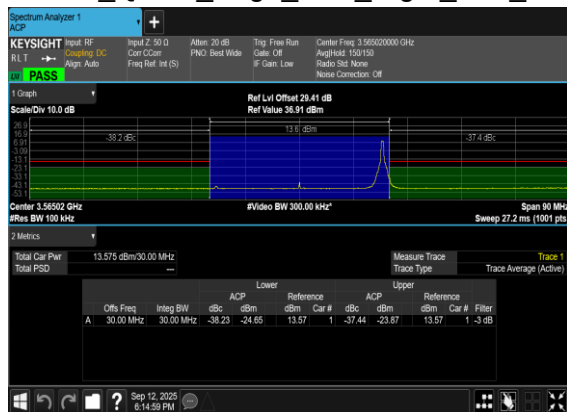
N48(30M)_DFT-s-OFDM_QPSK_Edge_1RB_Right_Low_CH
