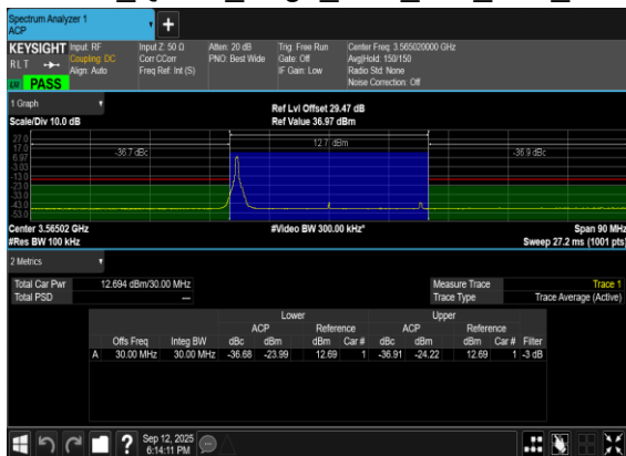
N48(30M)_DFT-s-OFDM_QPSK_Edge_1RB_Left_Low_CH
