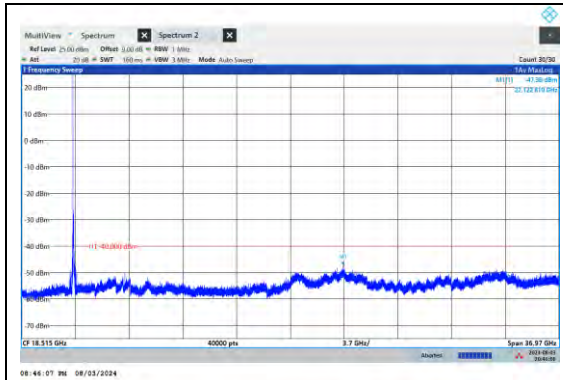
NTVN-N48-PC3-15-50-L-DFT-QPSK-Edge_1RB_ Left-Ant5-PASS
