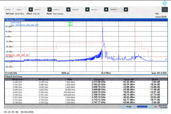
NTNV-N48-PC3-15-50-H-DFT-QPSK-Edge_1RB_ Left-Ant5-PASS
