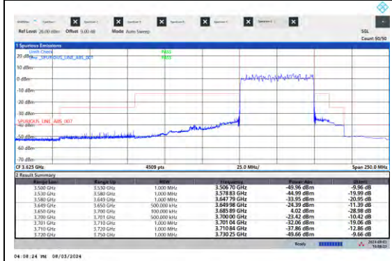
NTNV-N48-PC3-15-50-H-DFT-QPSK-Outer_Full-A nt5-PASS
