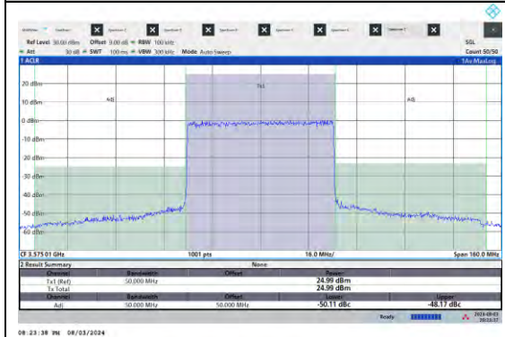
NTNV-N48-PC3-15-50-L-DFT-QPSK-Outer_Full-Ant5-PASS
