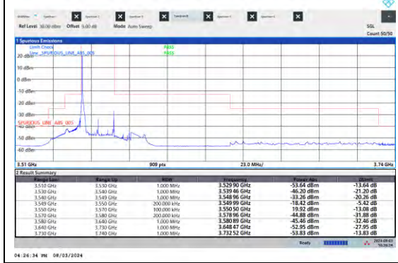
NTNV-N48-PC3-15-20-L-DFT-QPSK-Edge_1RB_Left-Ant5-PASS
