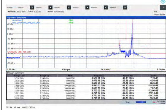
NTNV-N48-PC3-15-10-H-DFT-QPSK-Edge_1RB_Right-Ant5-PASS
