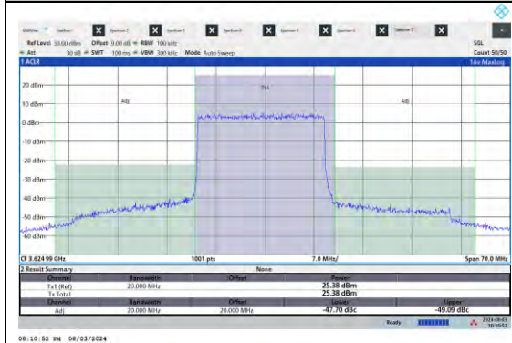
NTNV-N48-PC3-15-20-M-DFT-QPSK-Outer_Full-Ant5-PASS
