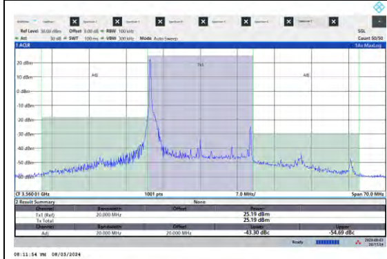
NTNV-N48-PC3-15-20-L-DFT-QPSK-Edge_1RB_ Left-Ant5-PASS
