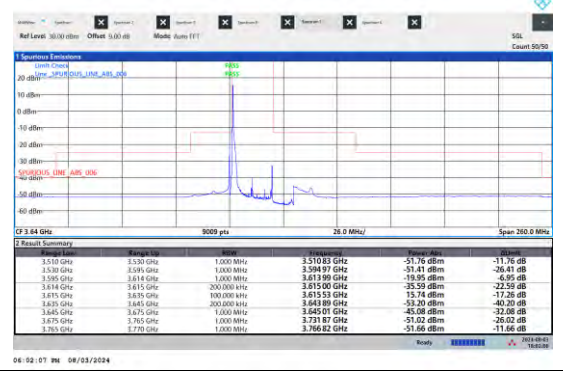
NTNV-N48-PC3-15-20-M-DFT-QPSK-Edge_1RB_Left-Ant5-PASS
