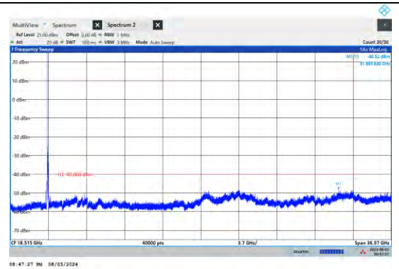
NTVN-N48-PC3-15-50-M-DFT-QPSK-Edge_1RB_ Left-Ant5-PASS
