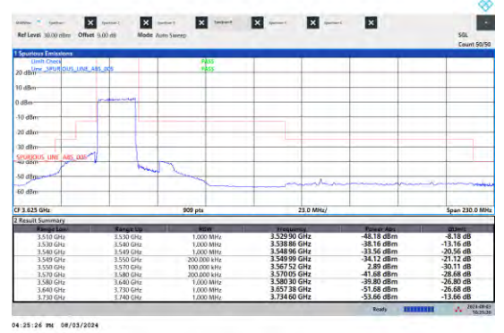
NTNV-N48-PC3-15-20-L-DFT-QPSK-Outer_Full-Ant5-PASS
