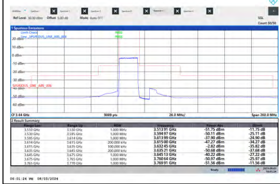
NTNV-N48-PC3-15-20-M-DFT-QPSK-Outer_Full-Ant5-PASS
