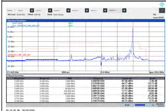
NTNV-N48-PC3-15-50-H-DFT-QPSK-Edge_1RB_ Right-Ant5-PASS
