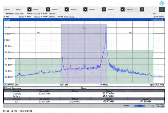
NTNV-N48-PC3-15-20-L-DFT-QPSK-Edge_1RB_ Right-Ant5-PASS
