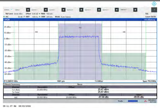
NTNV-N48-PC3-15-20-L-DFT-QPSK-Outer_Full-A nt5-PASS
