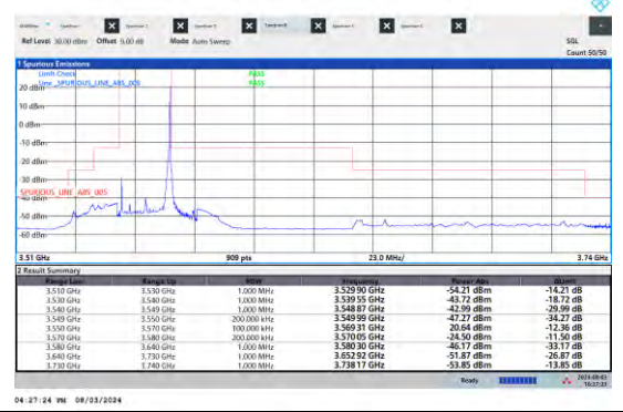
NTNV-N48-PC3-15-20-L-DFT-QPSK-Edge_1RB_Right-Ant5-PASS
