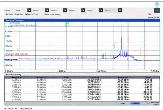
NTNV-N48-PC3-15-10-H-DFT-QPSK-Edge_1RB_Left-Ant5-PASS
