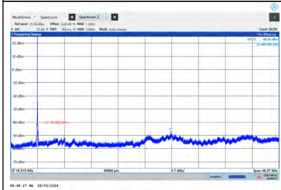
NTVN-N48-PC3-15-50-H-DFT-QPSK-Edge_1RB_ Left-Ant5-PASS
