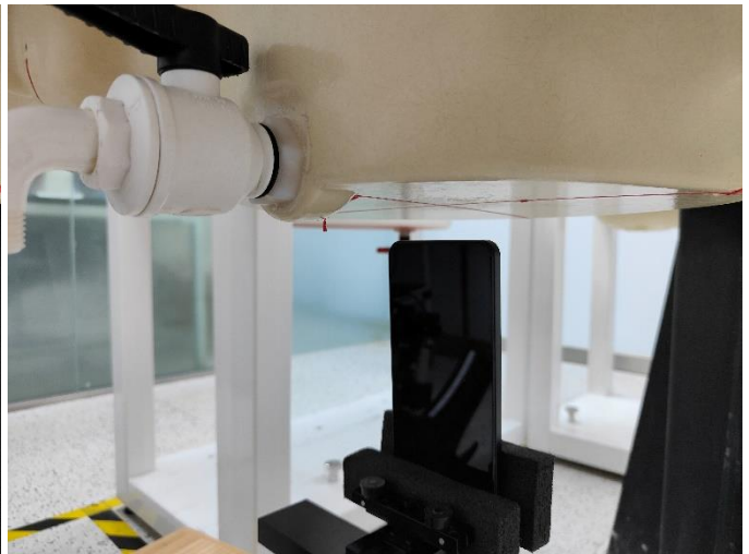
Bottom Side of EUT with 2.1 cm Gap (Body Mode)
