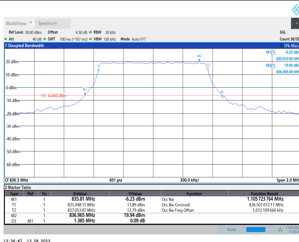
Band26-1.4MHz-16QAM-26915-6RB#0
