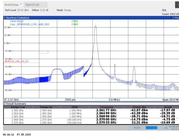
Band38-5MHz-QPSK-37775-25RB#0
