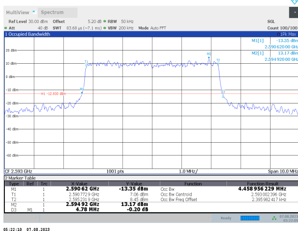
Band41-5MHz-16QAM-40620-25RB#0
