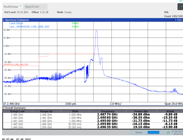
Band41-5MHz-QPSK-39675-25RB#0
