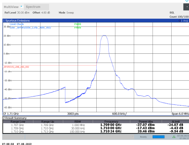
Band66-1.4MHz-QPSK-131979-6RB#0
