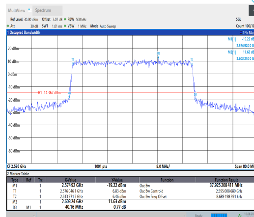
1-N38-PC3-30-40-M-8-CP-64QAM-Outer_Full-106@ @0-Ant1-37.925-40.160-≤40-PASS
