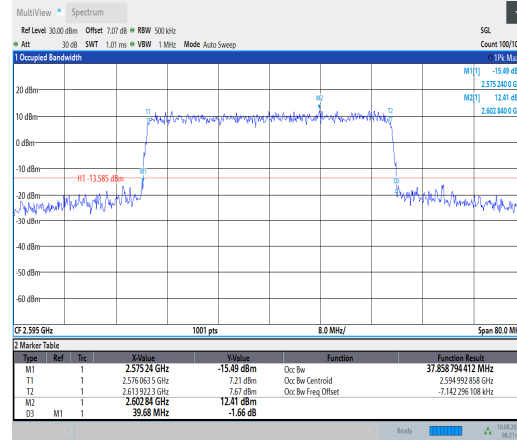
1-N38-PC3-30-40-M-6-CP-QPSK-Outer_Full-106@ 0-Ant1-37.859-39.680-≤40-PASS
