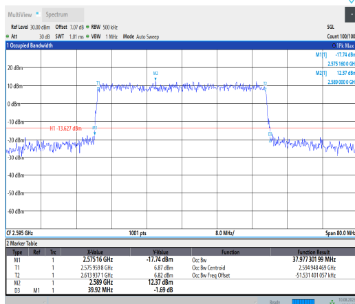
1-N38-PC3-30-40-M-7-CP-16QAM-Outer_Full-106@ 0-Ant1-37.977-39.920-≤40-PASS
