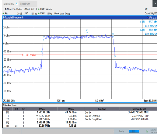
1-N38-PC3-30-40-M-5-DFT-256QAM-Outer_Full-100 @0-Ant1-35.677-37.360-≤40-PASS
