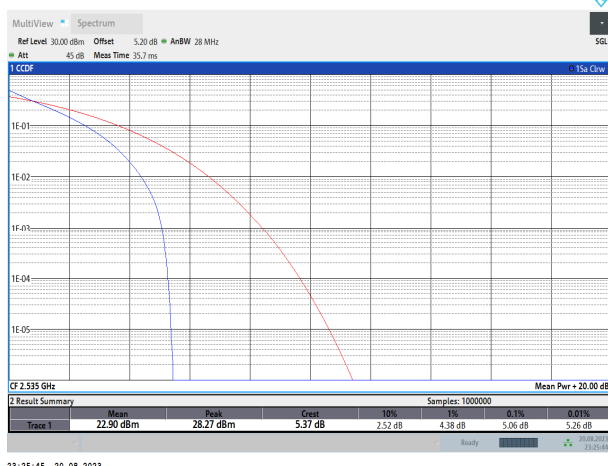
Band7-20MHz-QPSK-21100-100RB#0
