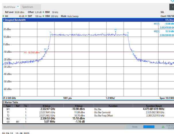
Band7-5MHz-16QAM-21100-25RB#0
