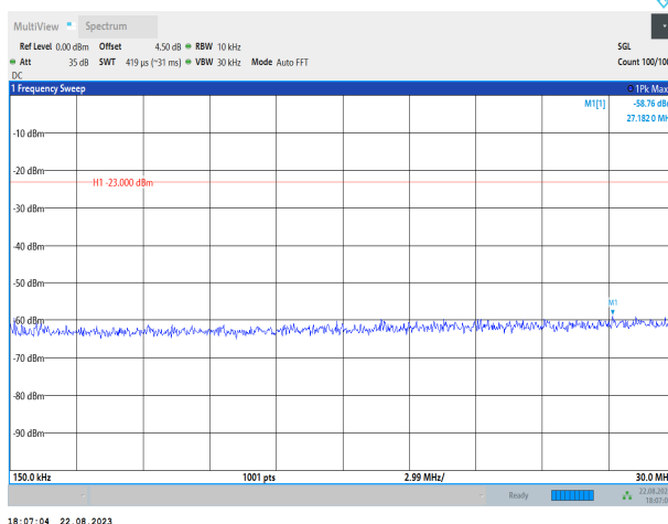
Band17-10MHz-QPSK-23780-1RB#0-Range2:0.15~30MHz
