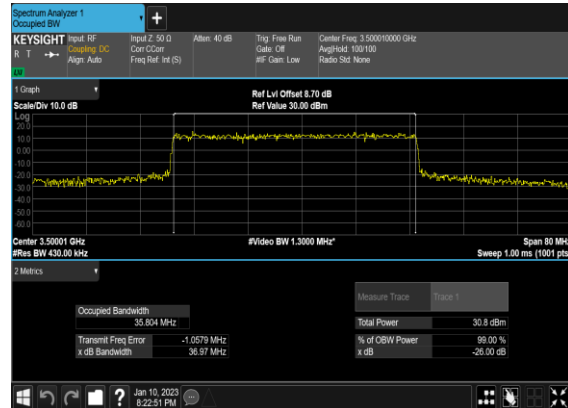
N77(40M)_DFT-s- OFDM_QPSK_Outer_Full_Mid_CH
