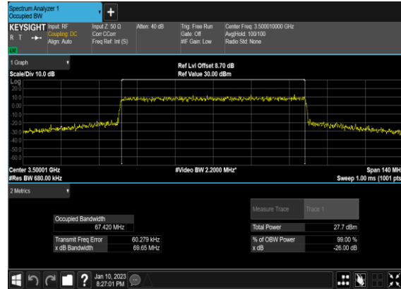
N77(70M)_CP-OFDM_16 QAM_Outer_Full_Mid_CH
