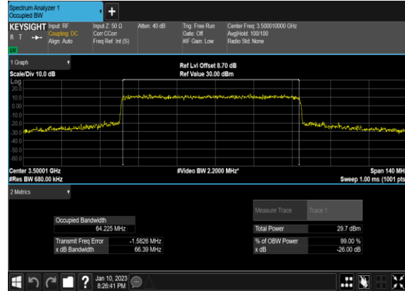
N77(70M)_DFT-s- OFDM_QPSK_Outer_Full_Mid_CH
