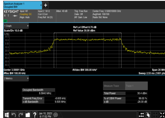
N77(10M)_DFT-s- OFDM_QPSK_Outer_Full_Mid_CH
