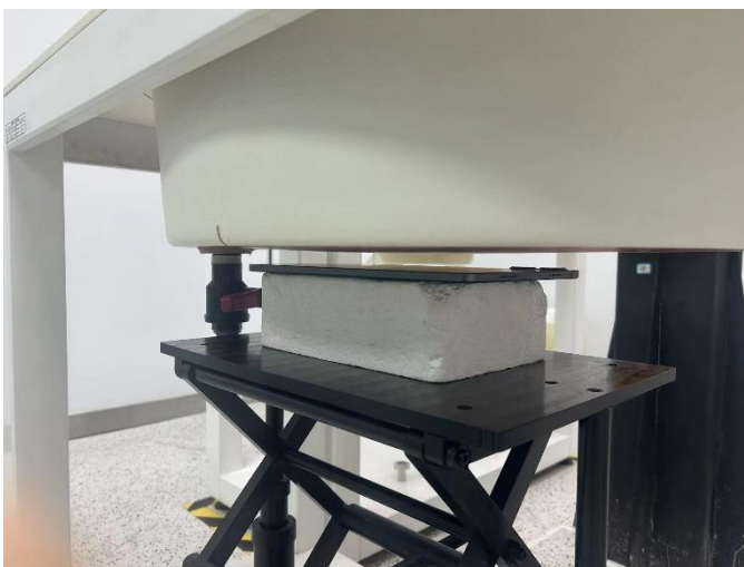
Rear Face of EUT with 1.6 cm Gap (Body Mode)
