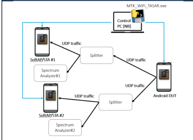
Figure 7.1.5 TA-SAR conducted power test setup for test scenarios 2 and 5 with Android DUT
