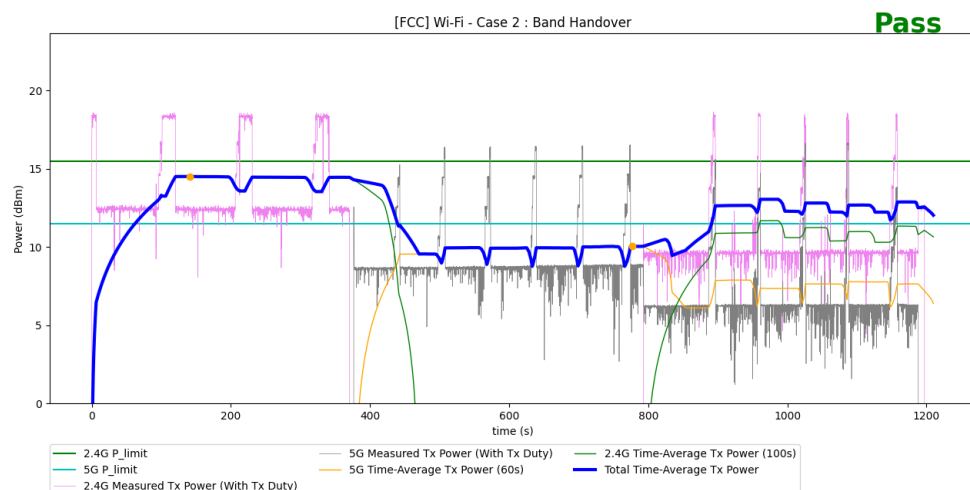
Figure 6-4 Time-averaged conducted TX power over time for test scenario 2
