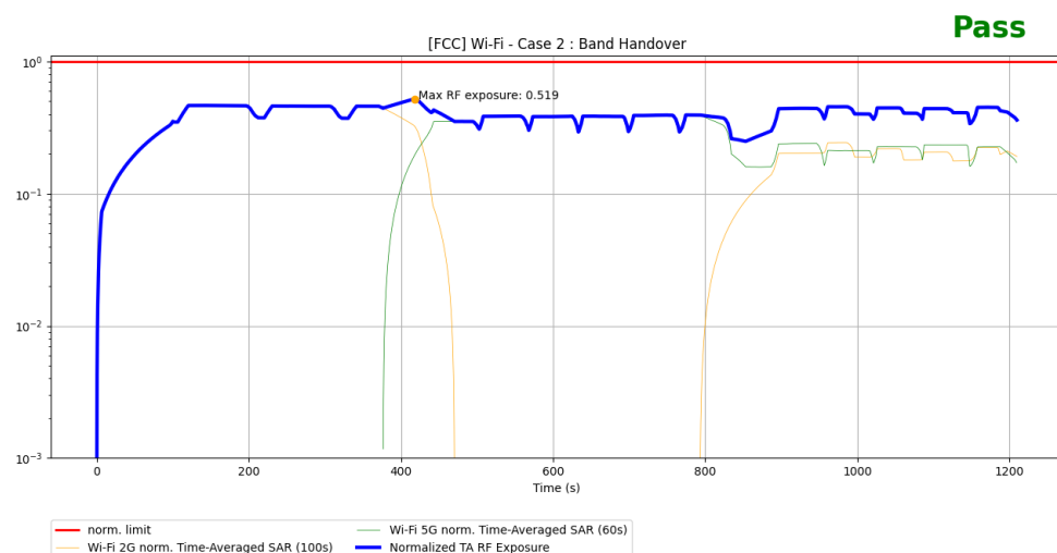
Figure 6-5 Normalized time-averaged SAR over time for test scenario 2
