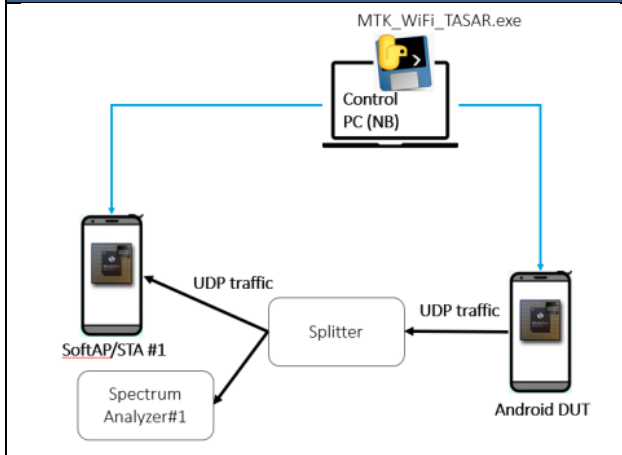
Figure 7.1.3 TA-SAR conducted power test setup for test scenarios 1 and 4 with Android DUT
