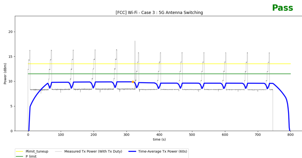
Figure 6-6 Time-averaged conducted TX power over time for test scenario 3
