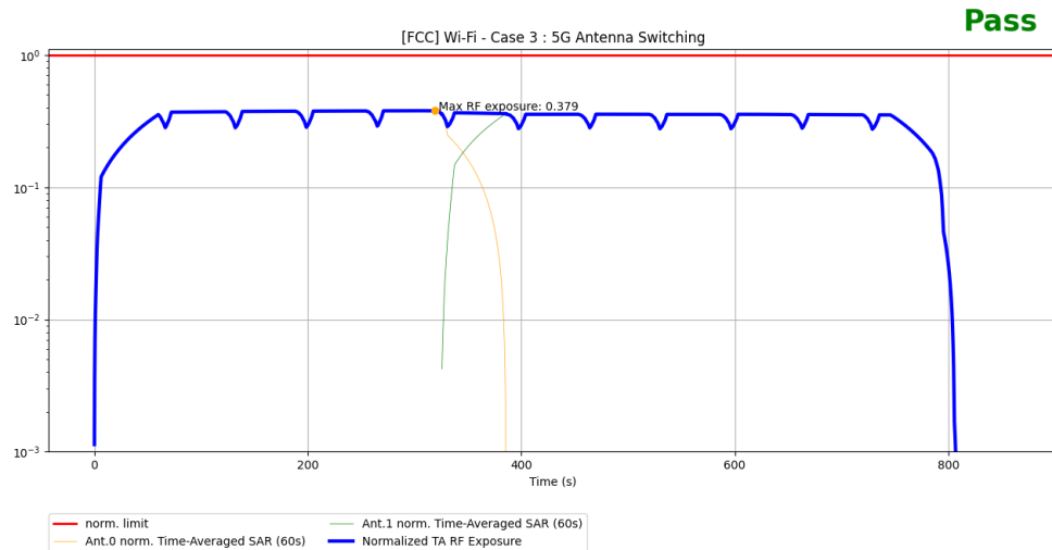
Figure 6-7 Normalized time-averaged SAR over time for test scenario 3
