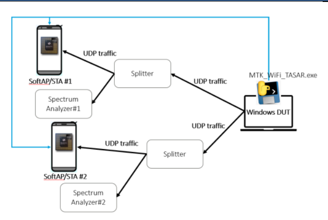
Figure 7.1.6 TA-SAR conducted power test setup for test scenarios 2 and 5 with Windows DUT
