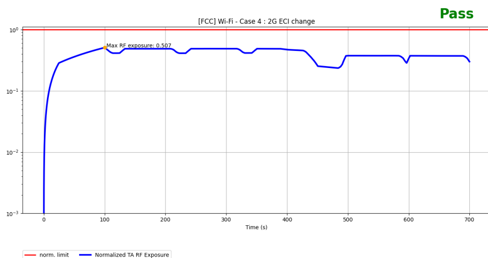
Figure 6-9 Normalized time-averaged SAR over time for test scenario 4
