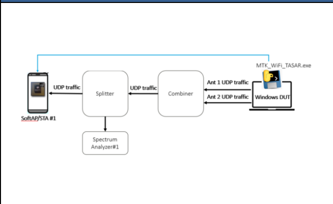
Figure 7.1.8 TA-SAR conducted power test setup for test scenario 3 with Windows DUT
