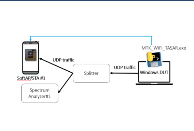
Figure 7.1.4 TA-SAR conducted power test setup for test scenarios 1 and 4 with Windows DUT
