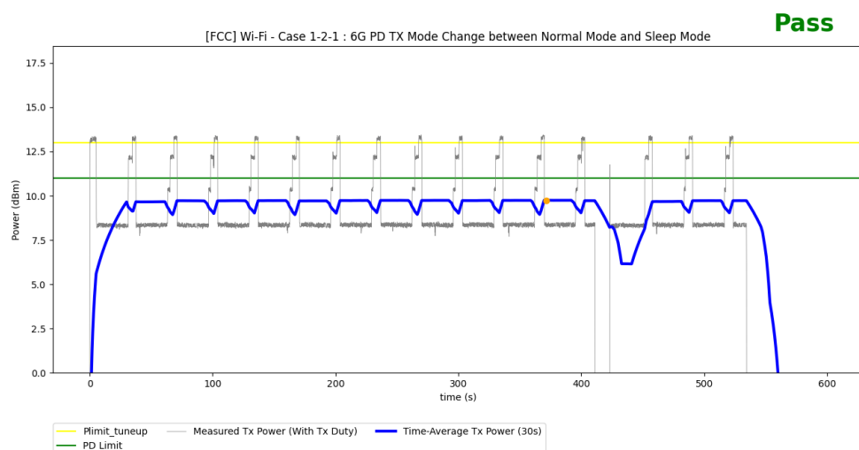
Figure 6-3 Time-averaged conducted TX power over time for test scenario 1
