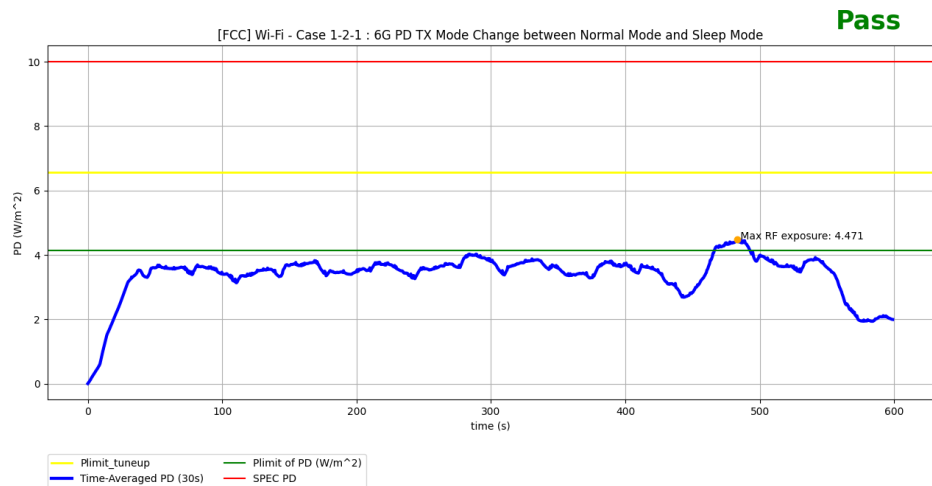
Figure 7-4 Time-averaged PD measurement result for Wi-Fi TA-SAR test scenario 1
