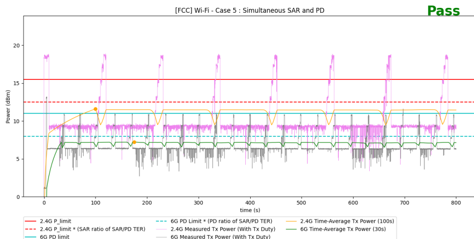
Figure 6-10 Time-averaged conducted TX power over time for test scenario 5
