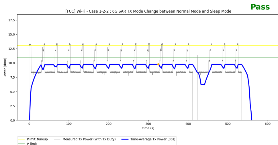
Figure 6-2 Time-averaged 6G conducted TX power over time for test scenario 1
