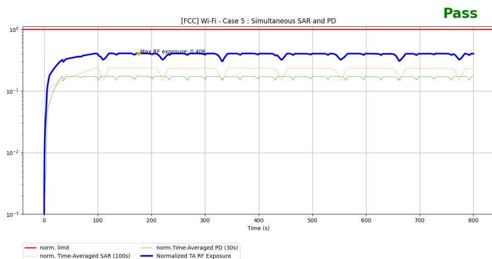
Figure 6-11 Normalized time-averaged SAR over time for test scenario 5
