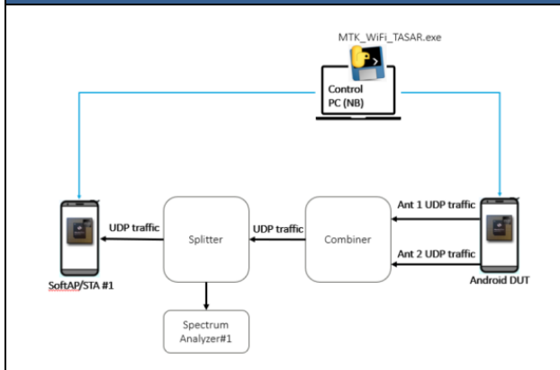
Figure 7.1.7 TA-SAR conducted power test setup for test scenario 3 with Android DUT
