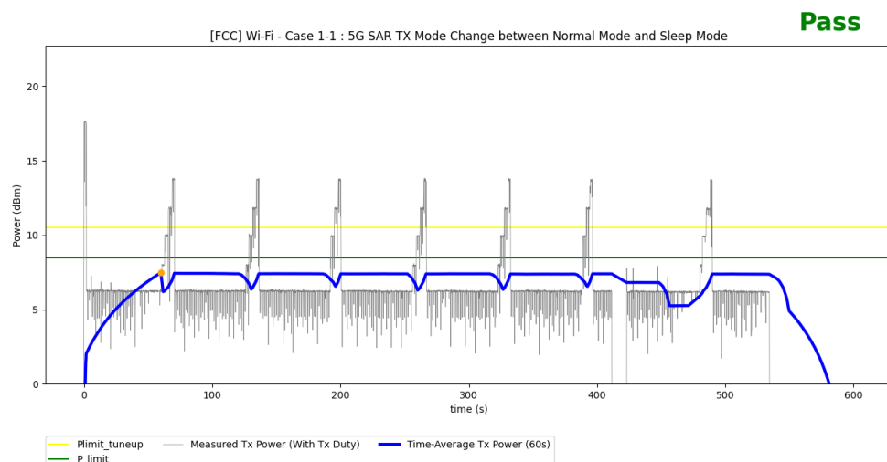
Figure 6-1 Time-averaged 5G conducted TX power over time for test scenario 1
