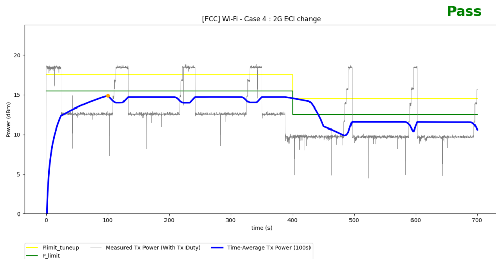
Figure 6-8 Time-averaged conducted TX power over time for test scenario 4
