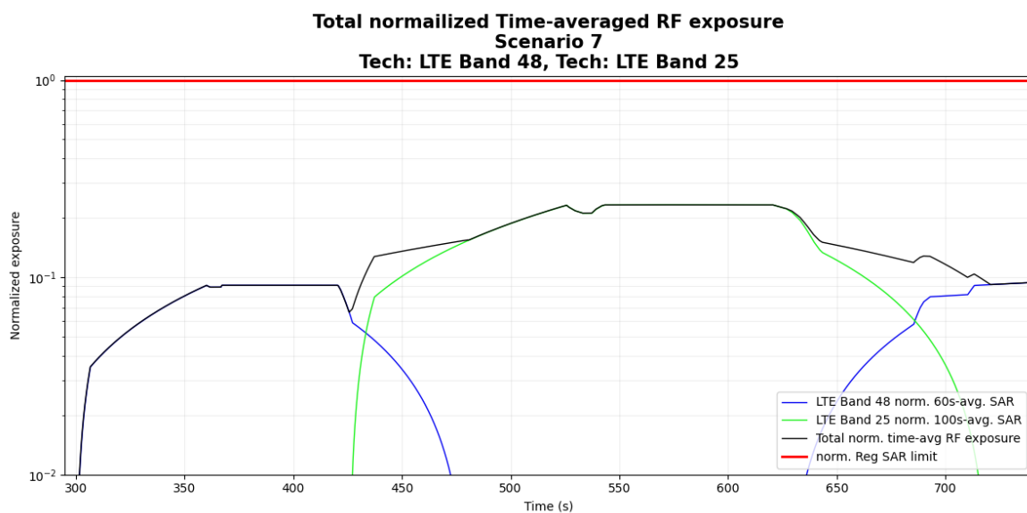
Figure 6- 24 Normalized time-averaged SAR
