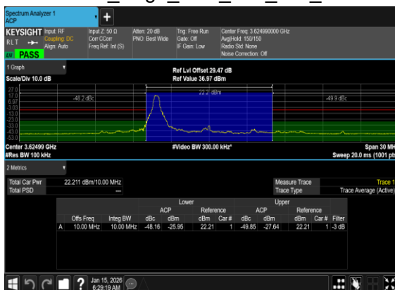
N48(10M)_DFT-s-OFDM_PI_2-BPSK_Edge_1RB_Left_Mid_CH
