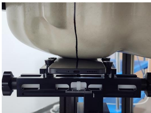
Photograph 1. Head, Right cheek, 0mm
