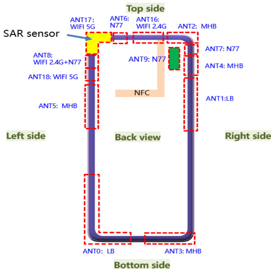
Photograph 9. Antenna position of EUT
