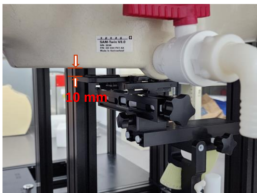
Photograph 5. Body, Back Side, 10mm
