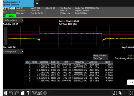
N77(100M)_DFT-s- OFDM_QPSK_Outer_Full_Mid_CH
