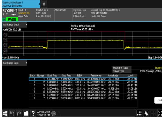
N77(100M)_DFT-s- OFDM_BPSK_Outer_Full_Mid_CH
