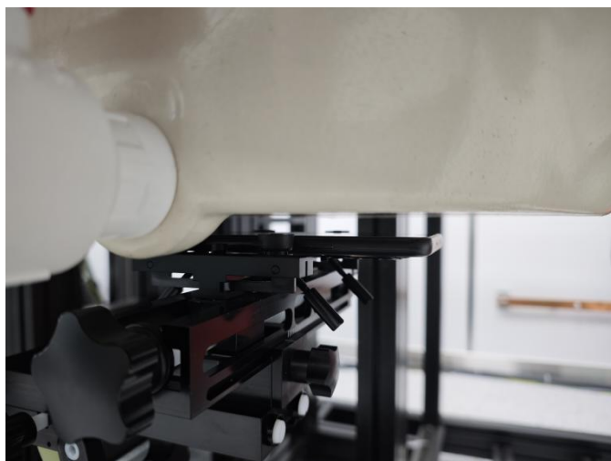
Front Face of EUT with 1 cm Gap (Body Mode)
