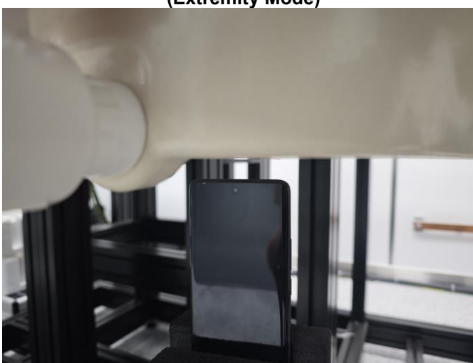
Top Side of EUT with 1.5 cm Gap (Extremity Mode)
