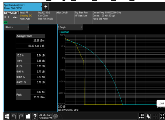
N2(20M)_DFT-s-OFDM_PI_2-BPSK_Edge_1RB_Left_Mid_CH
