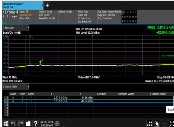
N38(25M)_DFT-s- OFDM_QPSK_Edge_1RB_Left_Low_CH
