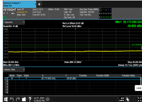
B4_N38(25M)_DFT-s-OFDM_QPSK_Edge_1RB_Left_Mid_CH
