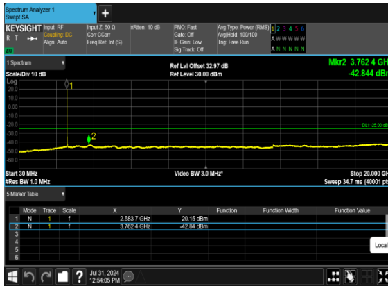
B4_N38(25M)_DFT-s-OFDM_BPSK_Edge_1RB_Left_Mid_CH
