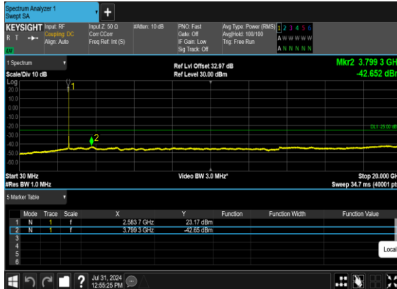
B4_N38(25M)_DFT-s-OFDM_QPSK_Edge_1RB_Left_Mid_CH
