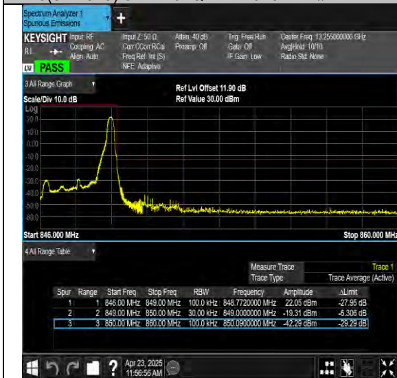
26(824-849)-3MHz-16QAM-26805-1RB#0-PASS
