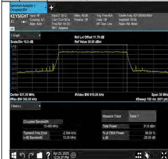
26(824-849)-15MHz-16QAM-26965-75RB#0-PASS
