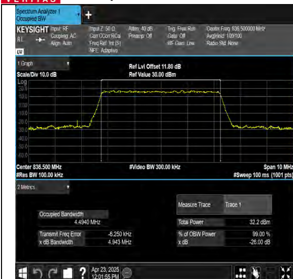
26(824-849)-5MHz-16QAM-26815-25RB#0-PASS
