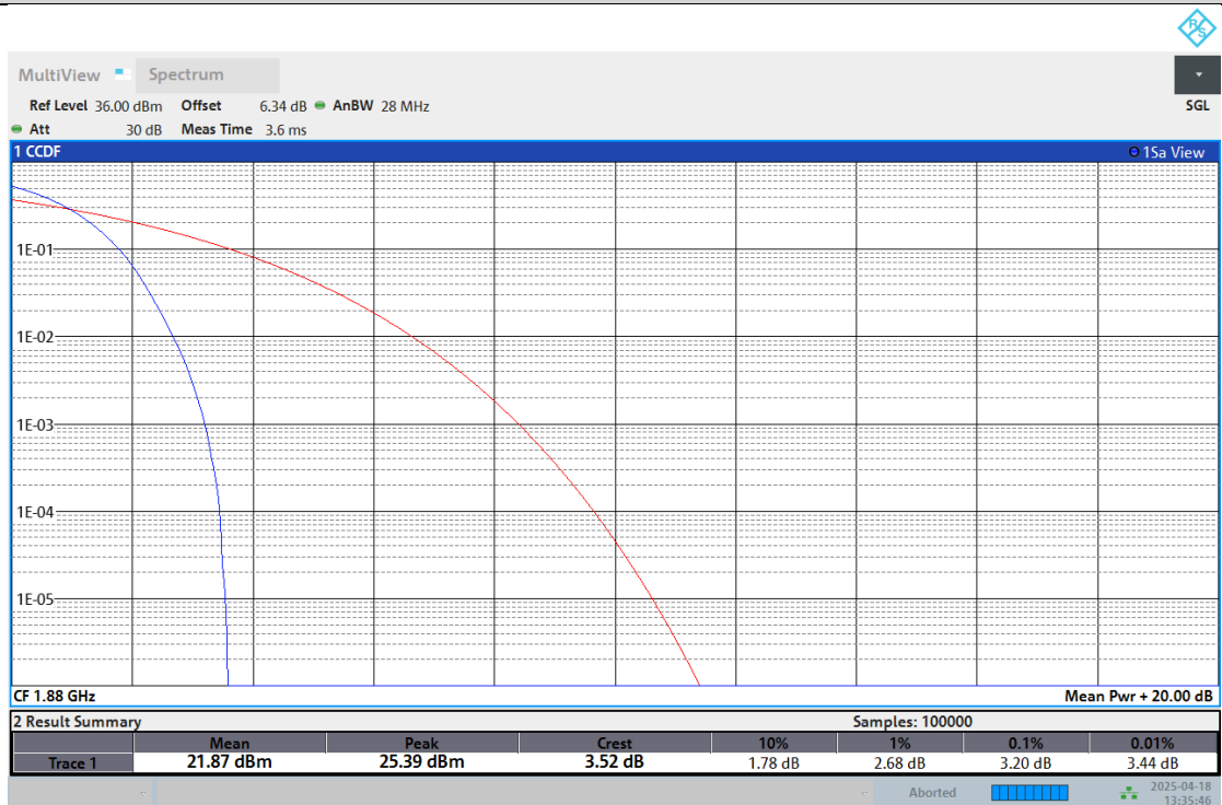
Band2-9538
