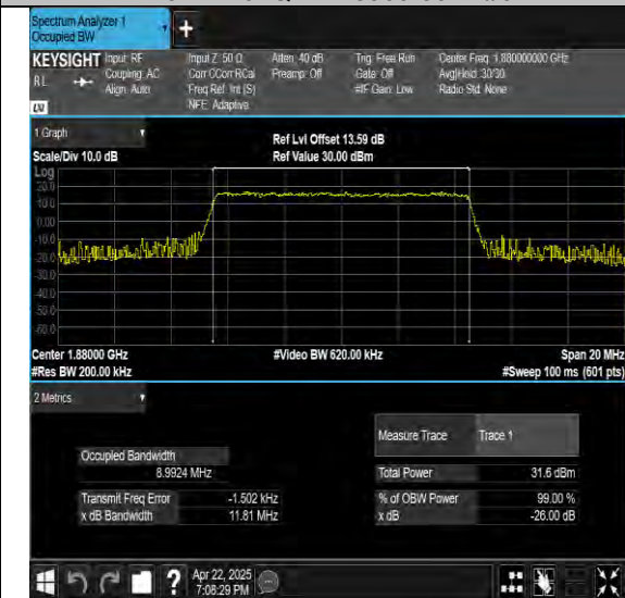
Band2-10MHz-16QAM-18650-50RB#0-PASS
