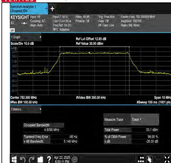
Band13-5MHz-16QAM-23205-25RB#0-PASS
