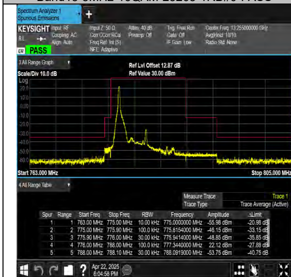
Band13-5MHz-16QAM-23255-1RB#24-PASS
