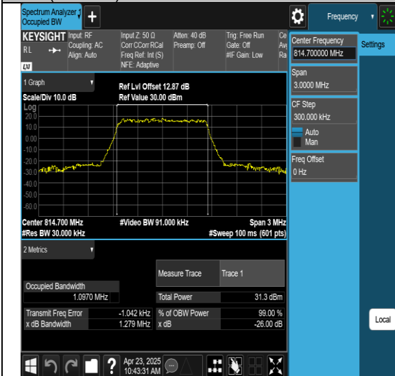
B26(814-824)-1.4MHz-16QAM-26783-6RB#0-PASS
