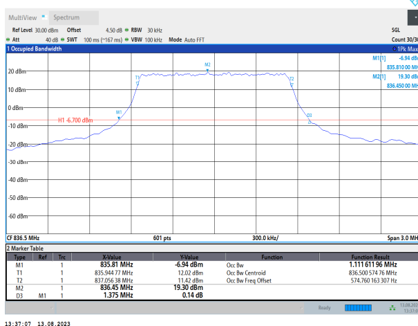
Band26-1.4MHz-16QAM-26915-6RB#0
