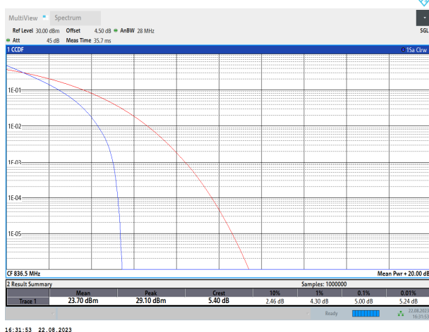
Band26-15MHz-QPSK-26915-75RB#0
