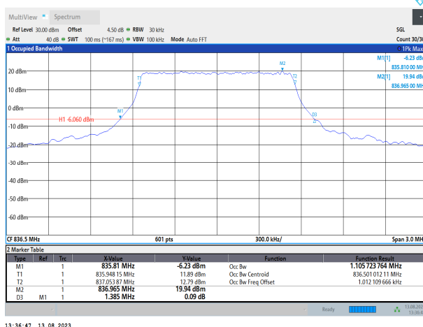
Band26-1.4MHz-16QAM-26915-6RB#0
