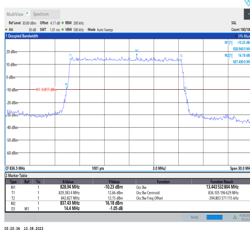
1-N5-PC3-15-15-M-2-DFT-PI2BPSK-Outer_Full-75@ 0-Ant1-13.444-14.400-≤15-PASS
