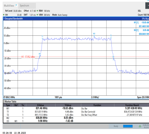
1-N5-PC3-15-10-M-9-CP-256QAM-Outer_Full-52@0- Ant1-9.281-9.980-≤10-PASS
