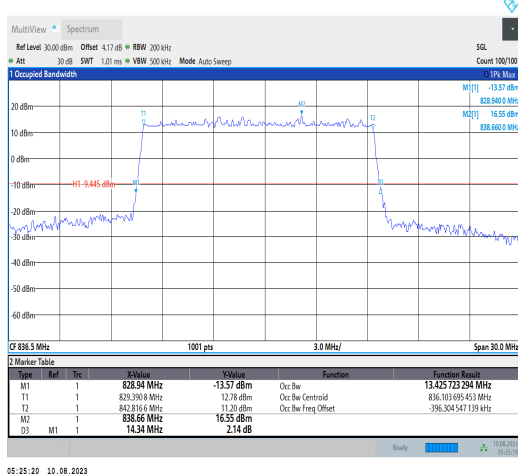
1-N5-PC3-15-15-M-1-DFT-QPSK-Outer_Full-75@0- Ant1-13.426-14.340-≤15-PASS
