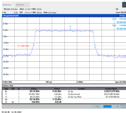
1-N5-PC3-15-10-M-8-CP-64QAM-Outer_Full-52@0 -Ant1-9.256-9.840-≤10-PASS
