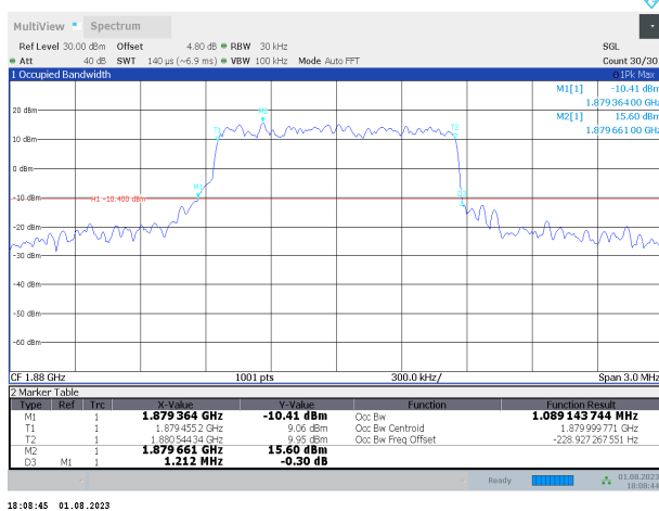
Band2-1.4MHz-16QAM-18900-6RB#0
