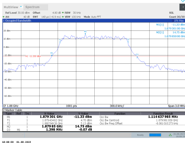
Band2-1.4MHz-16QAM-18900-6RB#0
