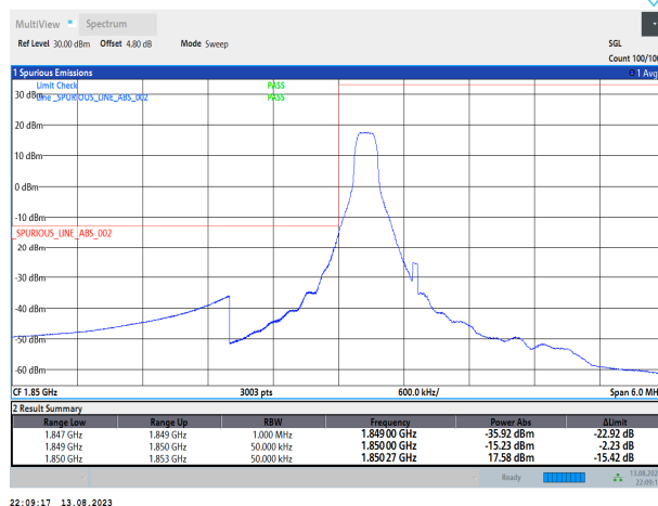
Band2-1.4MHz-QPSK-18607-6RB#0
