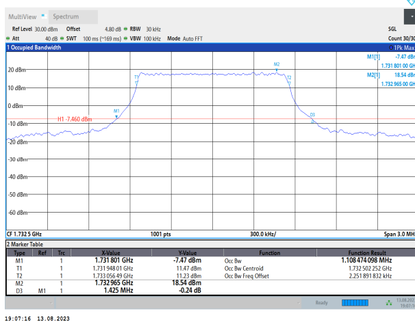
Band4-1.4MHz-16QAM-20175-6RB#0
