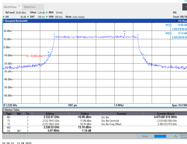
Band7-5MHz-16QAM-21100-25RB#0
