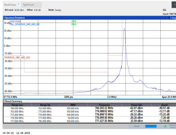
Band13-5MHz-QPSK-23205-25RB#0
