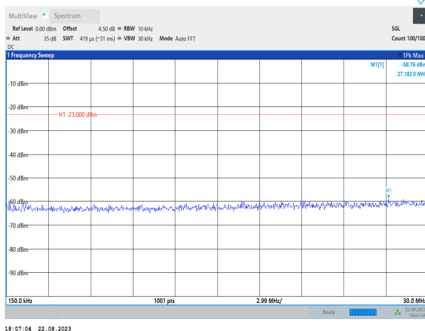
Band17-10MHz-QPSK-23780-1RB#0-Range2:0.15~30MHz
