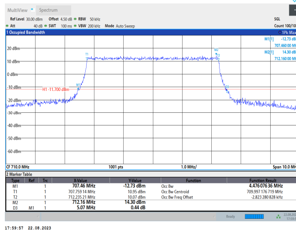
Band17-5MHz-16QAM-23790-25RB#0
