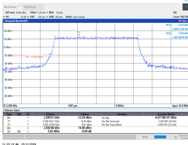
Band41-5MHz-16QAM-40620-25RB#0
